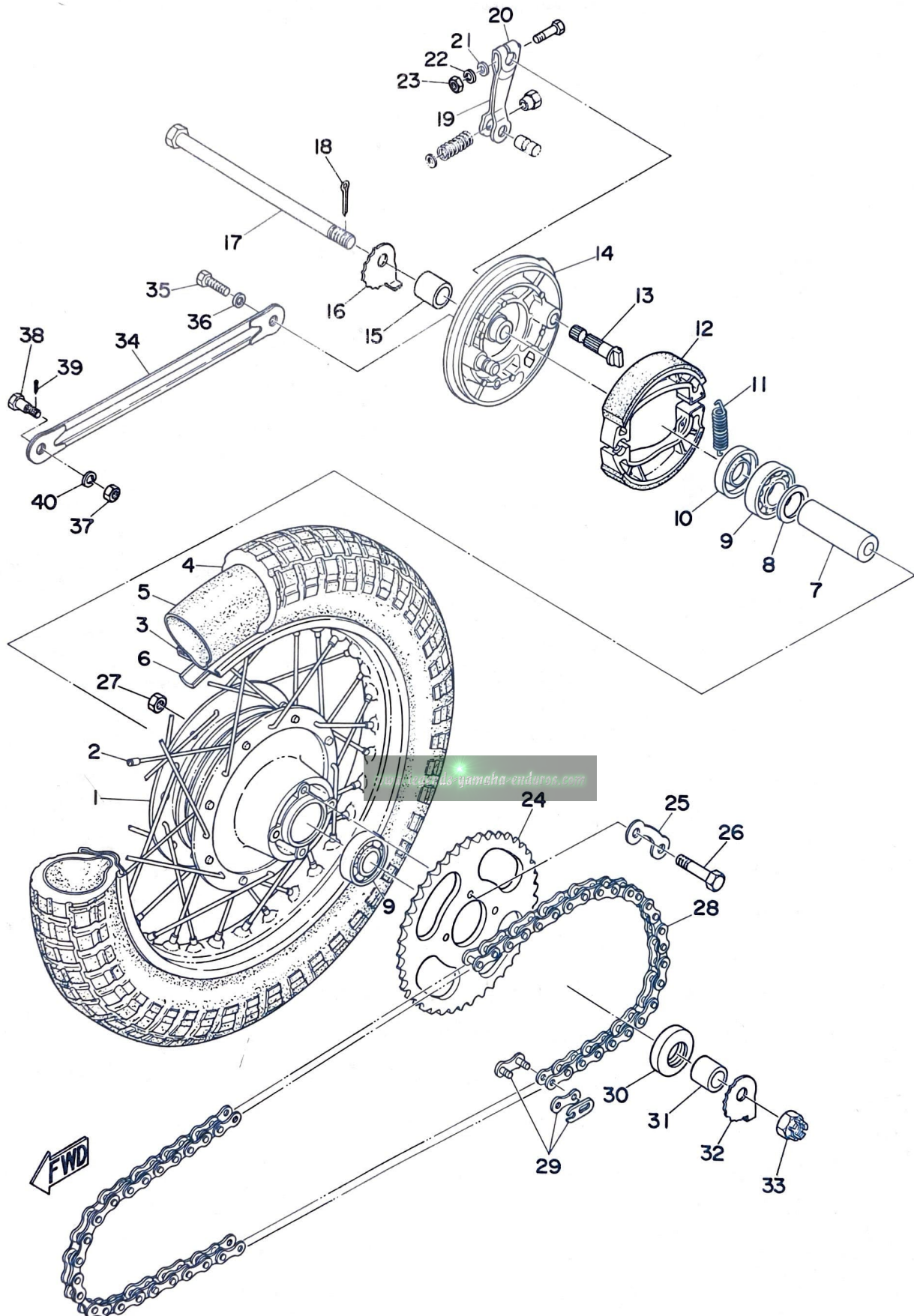
Fig. 25 REAR WHEEL
