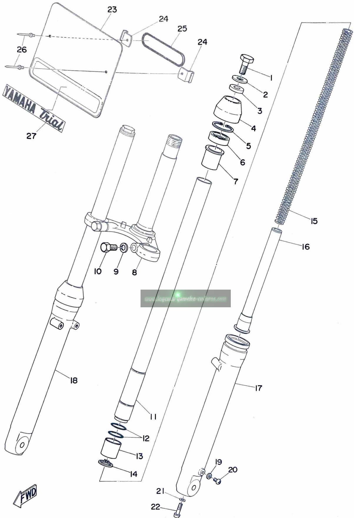
Fig. 18 FRONT FORK
