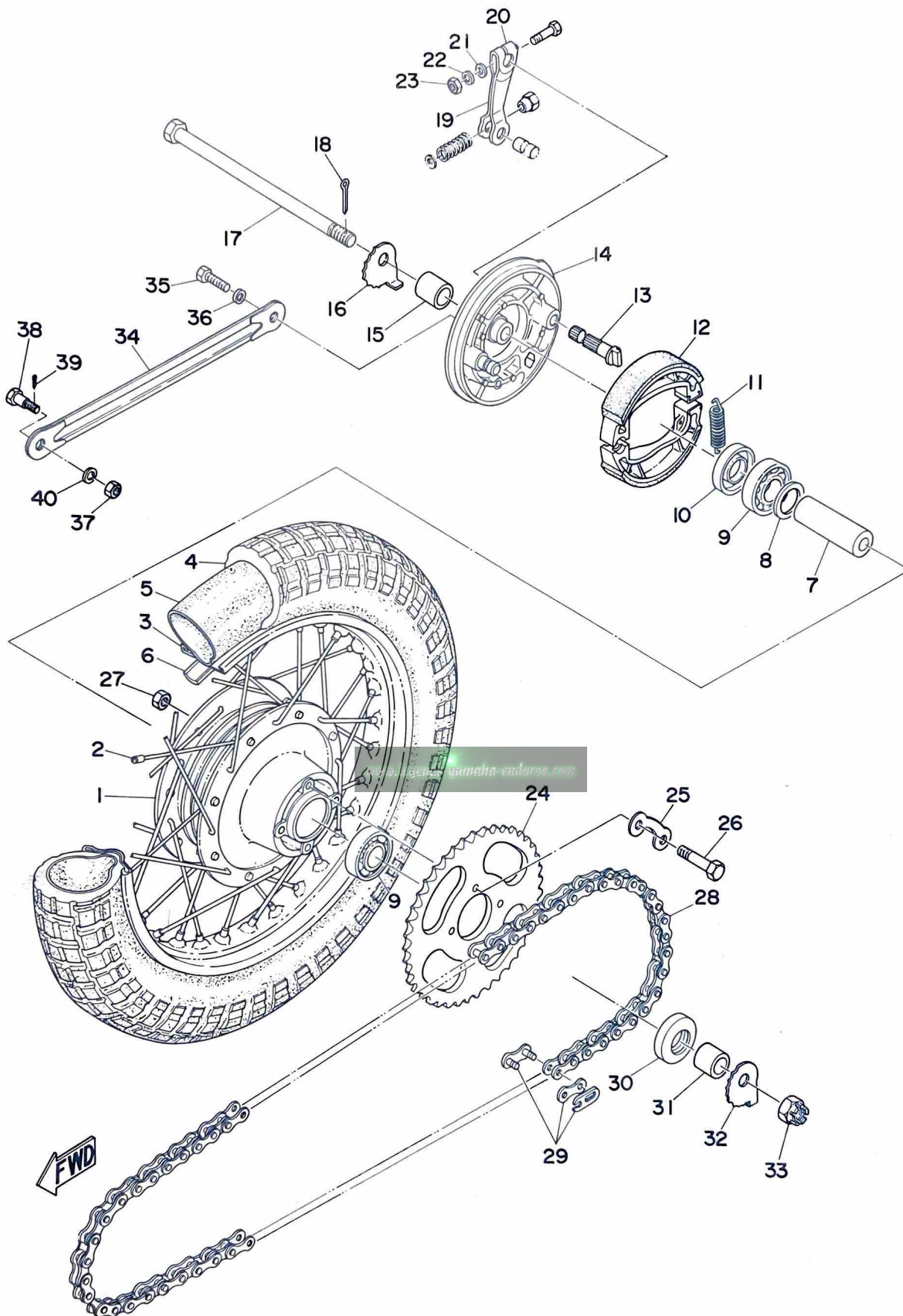
Fig. 25 REAR WHEEL
