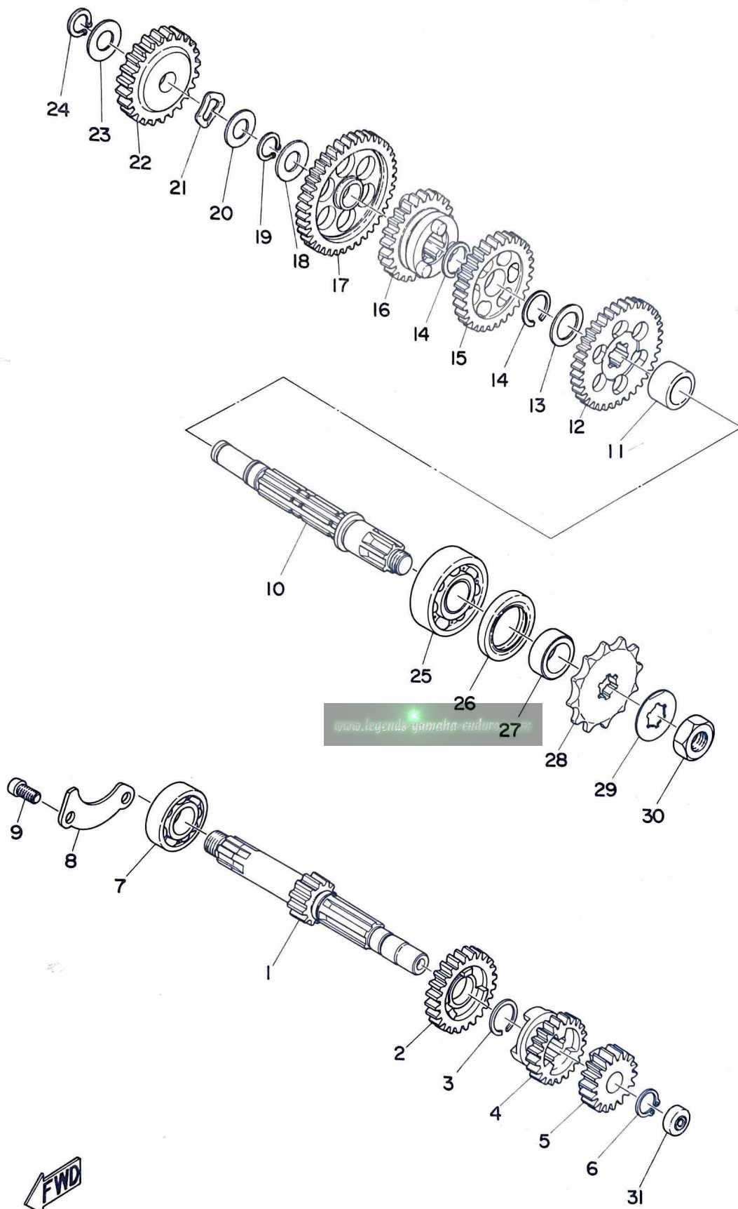
Fig. 5 TRANSMISSION
