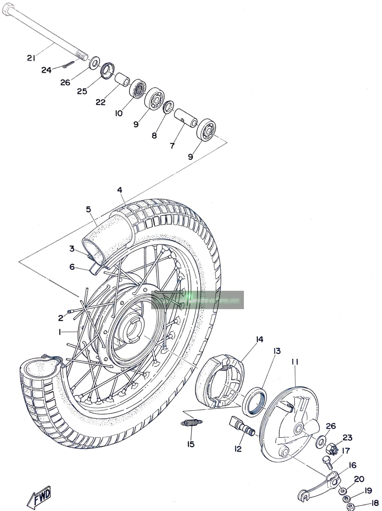
Fig. 24 FRONT WHEEL
