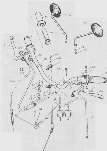
Figure No. 15 1A1.19.00.00 - HANDLE BAR
