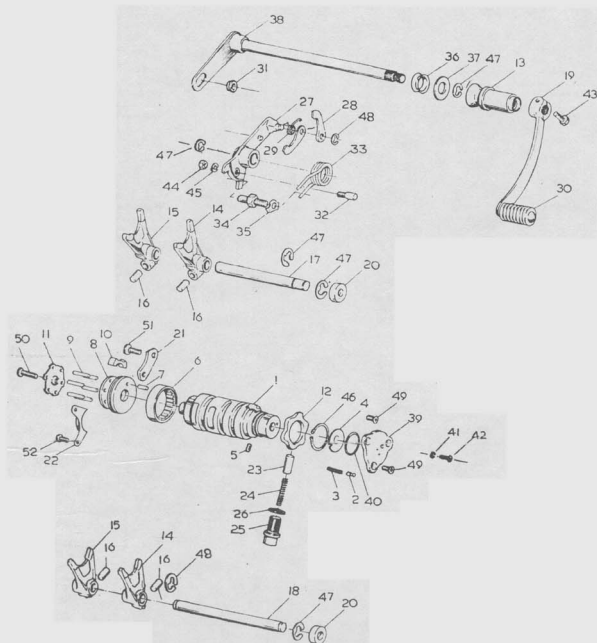
Figure No. 38 1A1.60.00.00 - SHIFTER
