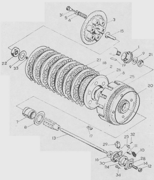
Figure No. 35 1 A1 57 00 00 - CLUTCH
