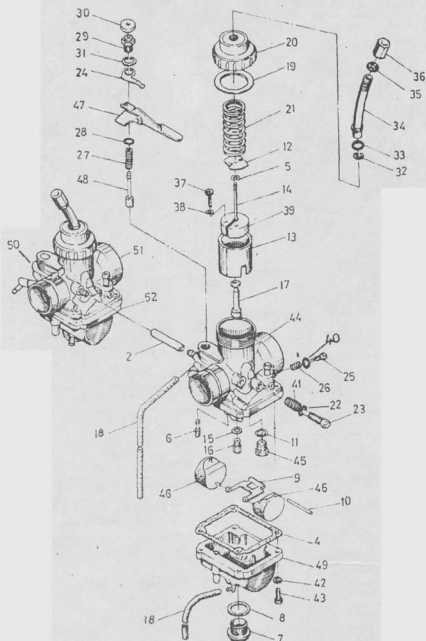
Figure No. 41 1A1.65.00.00 - CARBURETTOR ASSEMBLY
