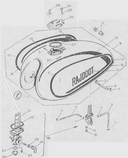
Fig:re No. 6 1 A1 07 00 00 - FUEL TANK
