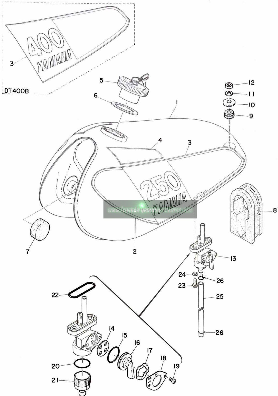
Fig. 26 FUEL TANK
