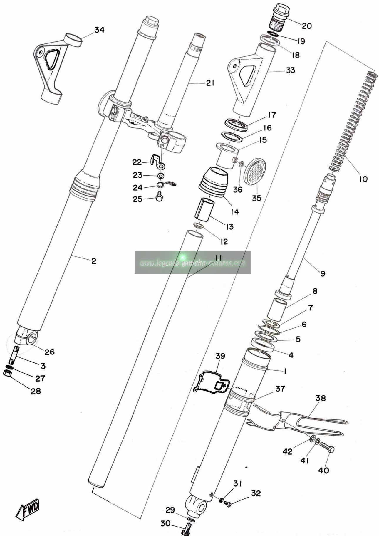
Fig. 23 FRONT FORK
