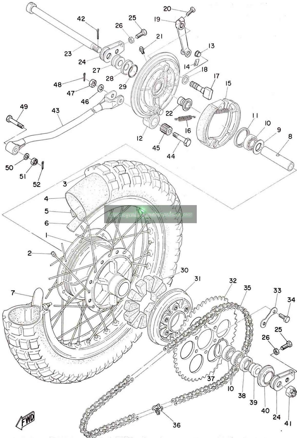
Fig. 30 REAR WHEEL
