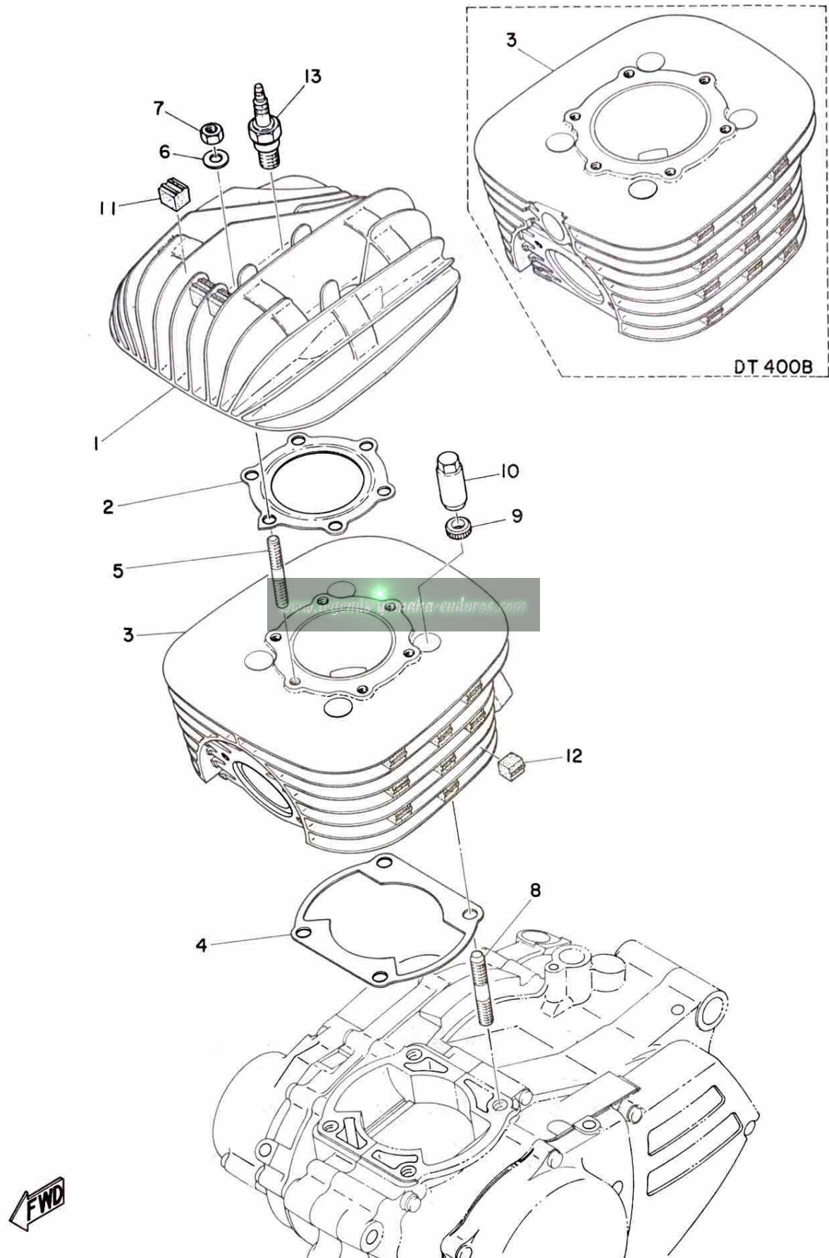
Fig. 1 CYLINDER HEAD · CYLINDER
