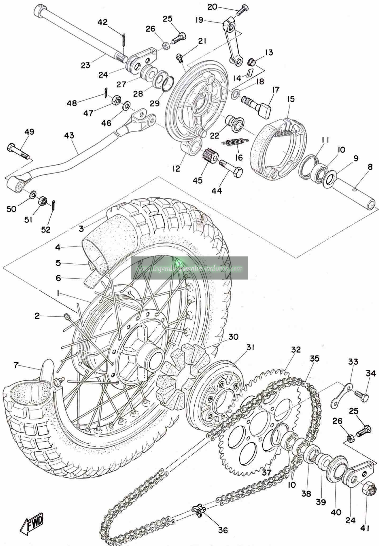
Fig. 30 REAR WHEEL
