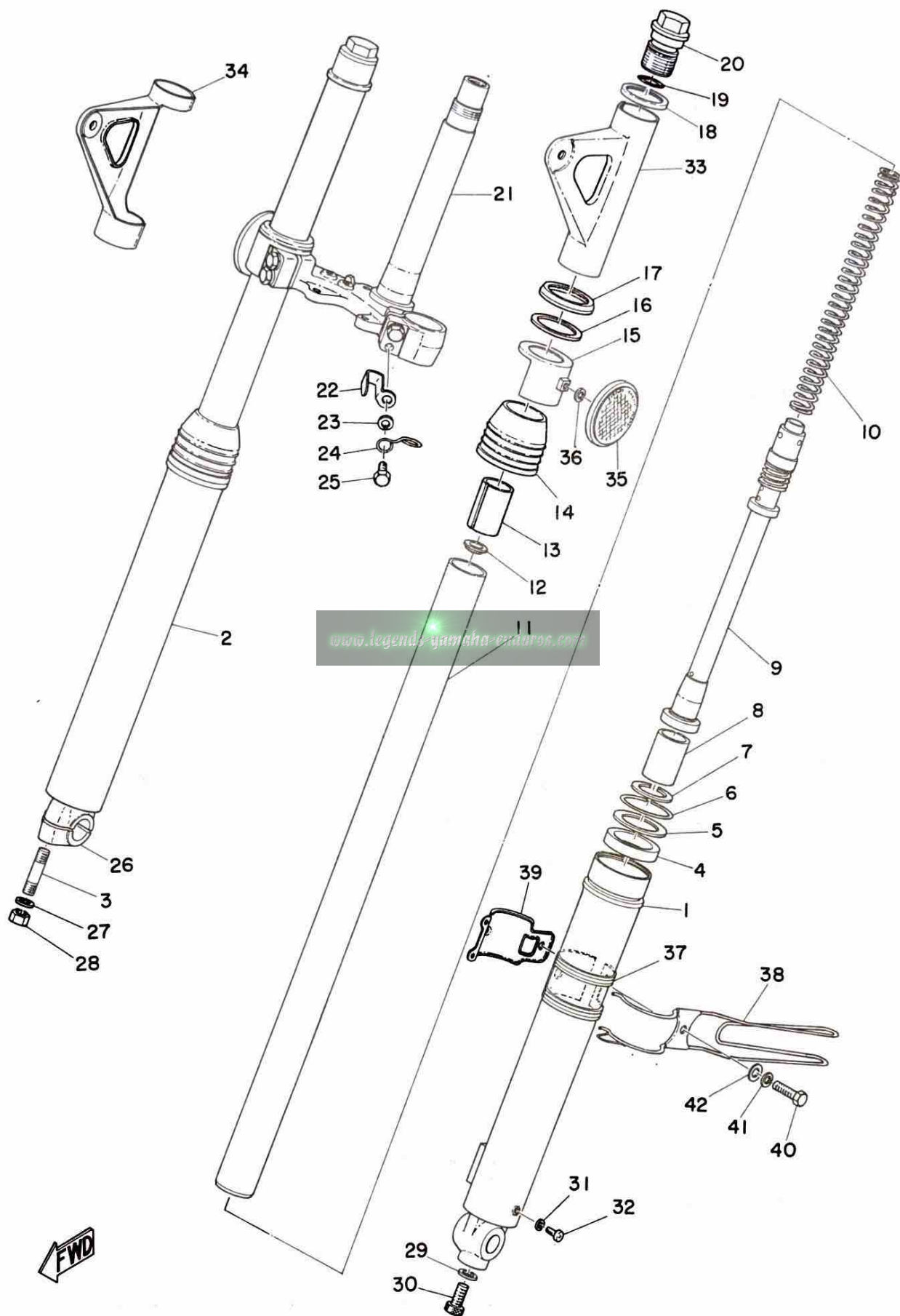
Fig. 23 FRONT FORK
