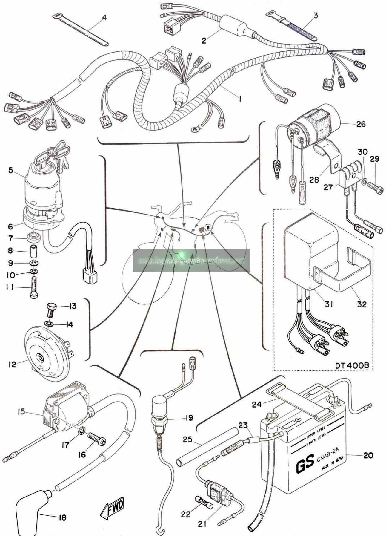
Fig. 35 ELECTRICAL
