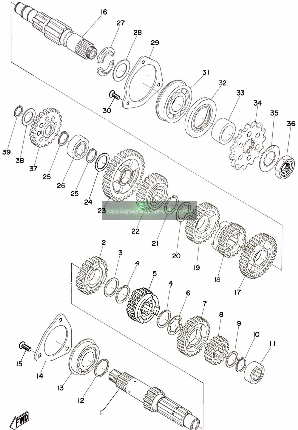
Fig. 6 TRANSMISSION
