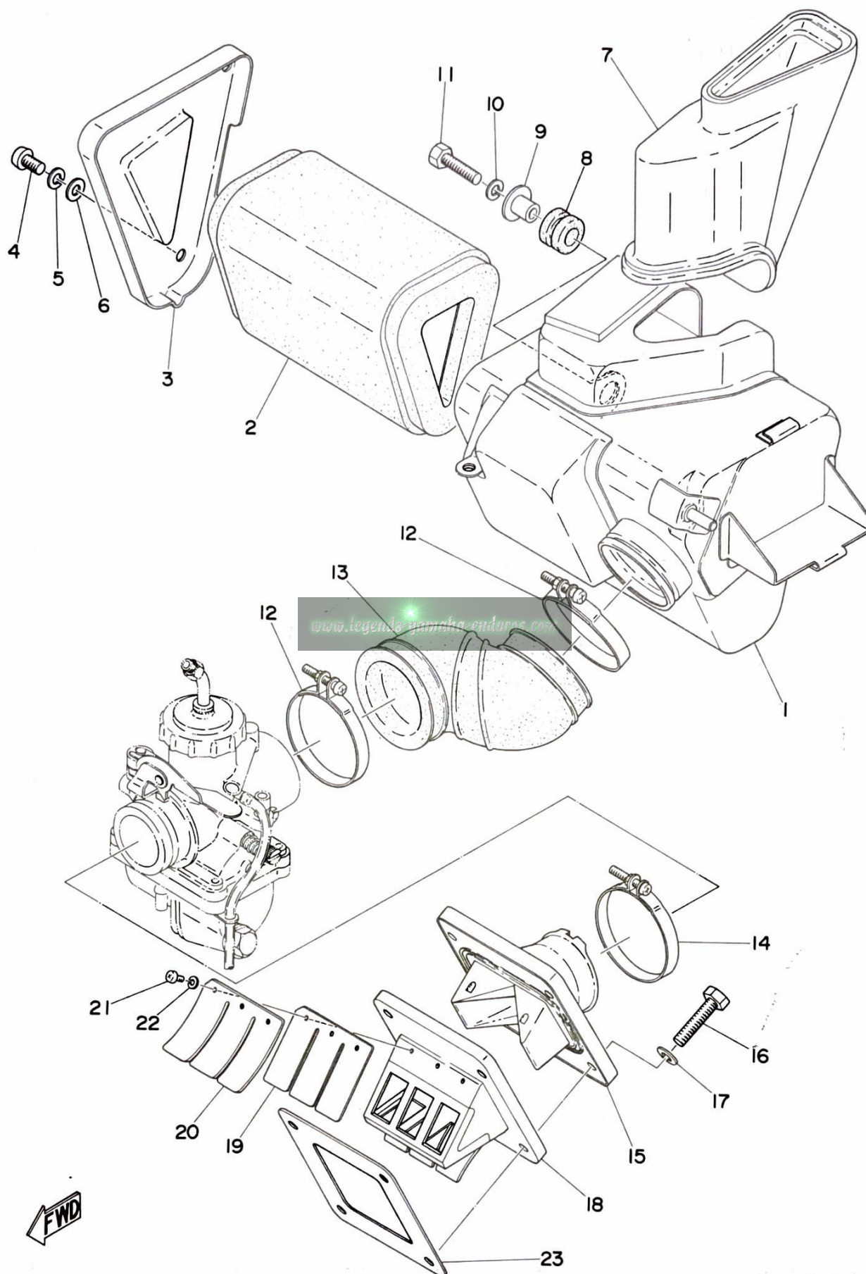
Fig. 12 INTAKE
