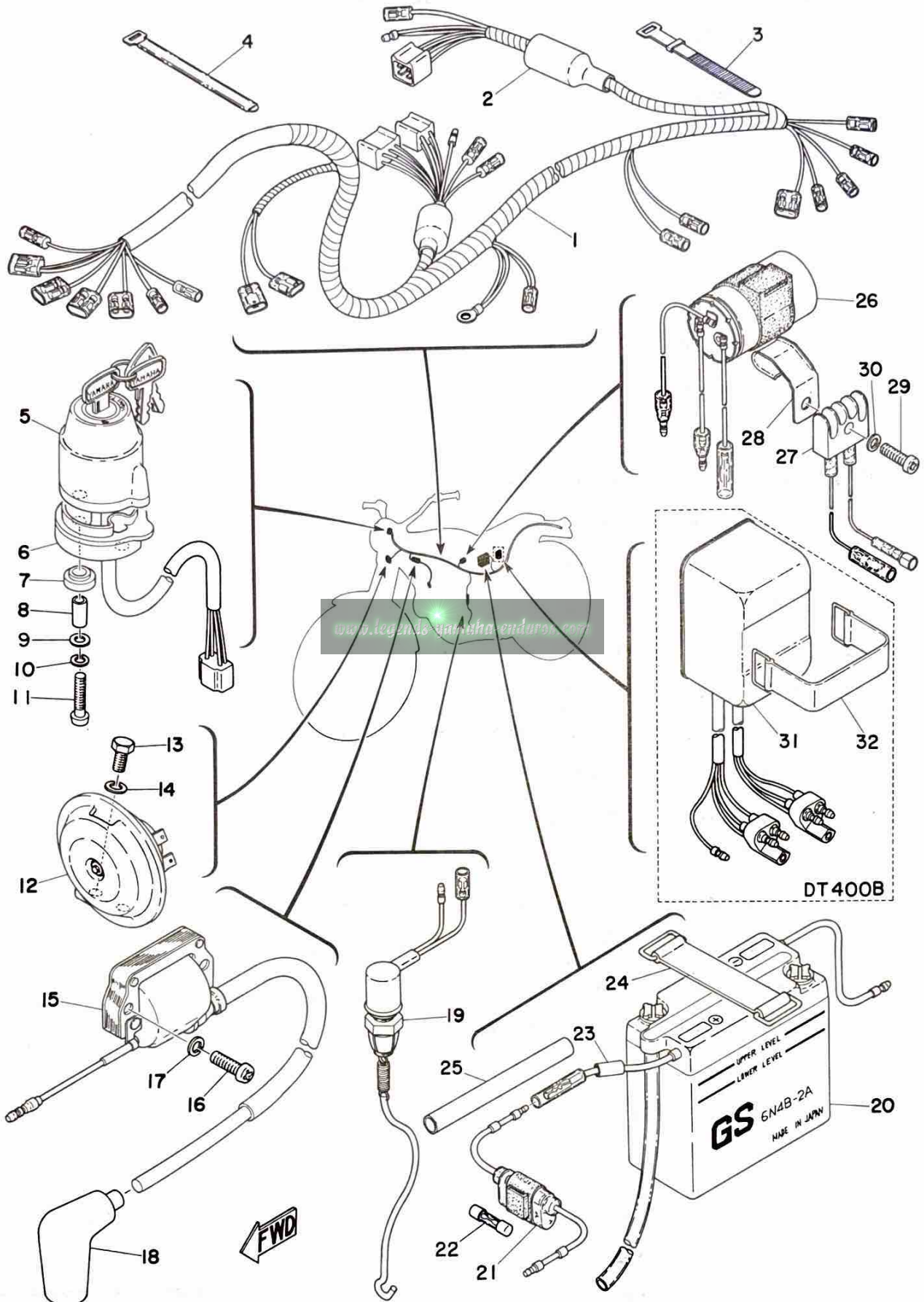
Fig. 35 ELECTRICAL
