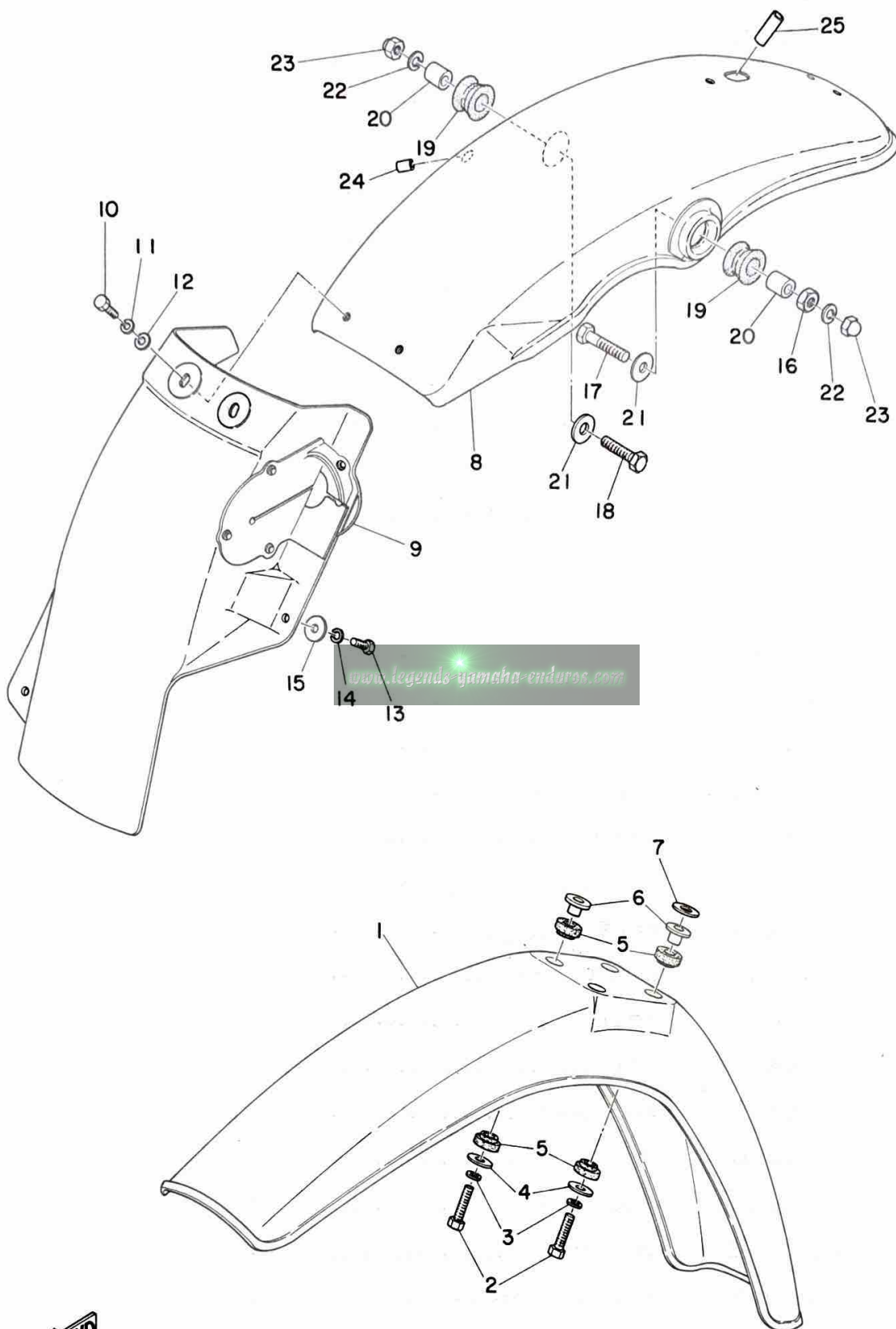
Fig. 22 FRONT FENDER · REAR FENDER
