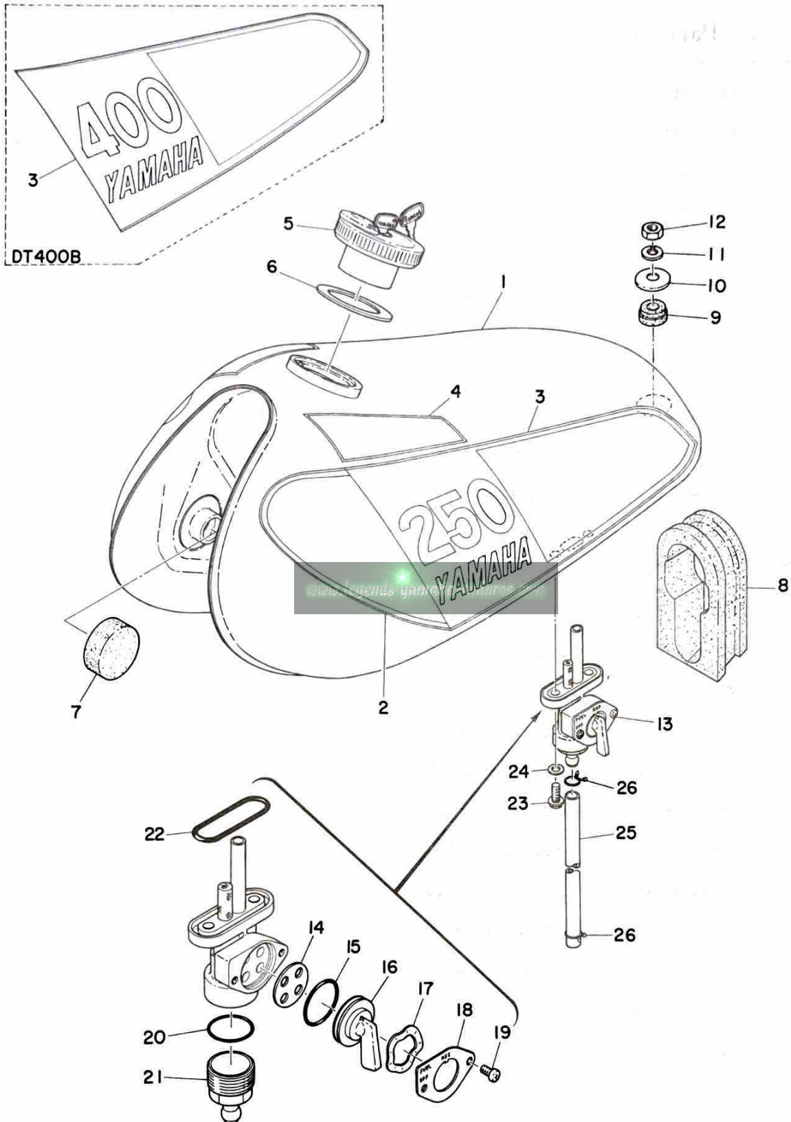
Fig. 26 FUEL TANK
