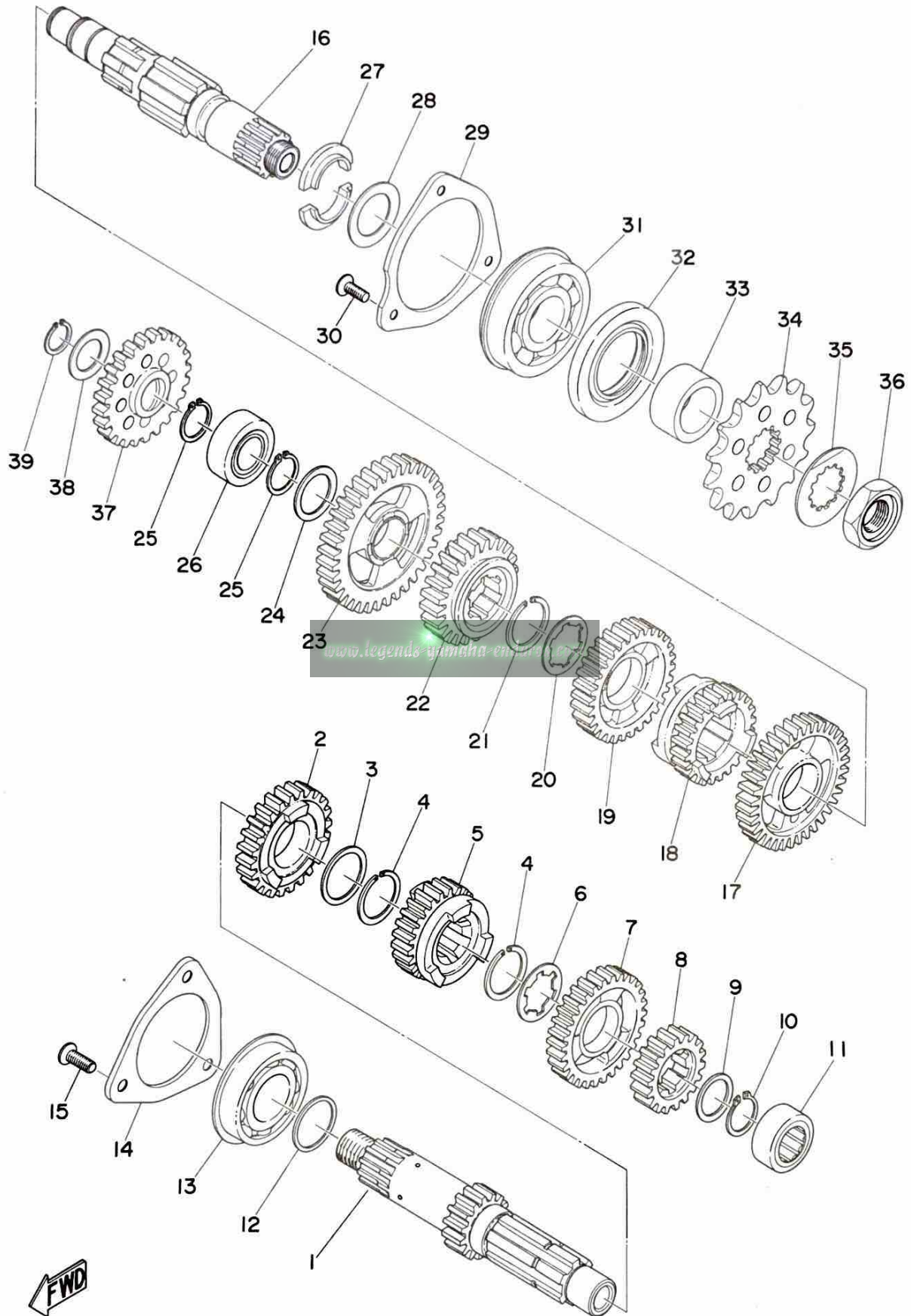
Fig. 6 TRANSMISSION
