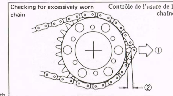
1. Tirer 2. 1/2 dent
