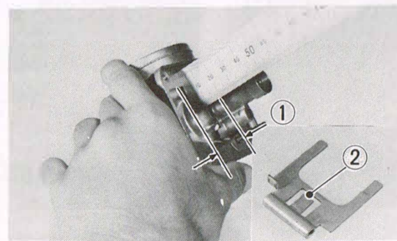
1. Float level 2. Tang
