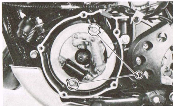
1. Base screw
