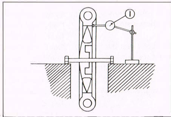
1. Dial gauge
