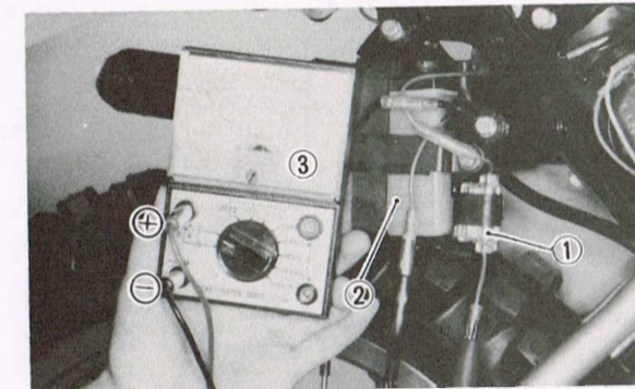
1. Fuse 2. Battery 3. Set the tester in "DC. A-5" position.
