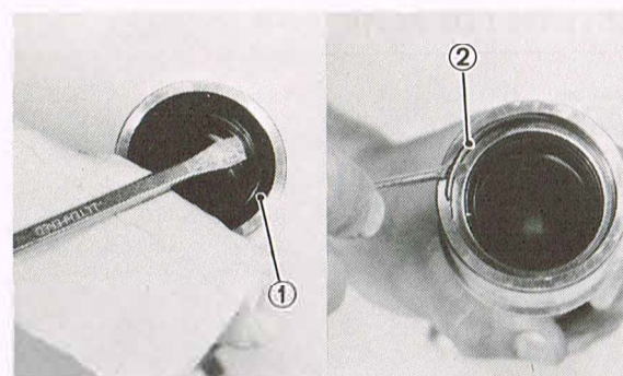
1. Dust seal 1. Joint anti-poussière 2. Snap ring 2. Circlip
