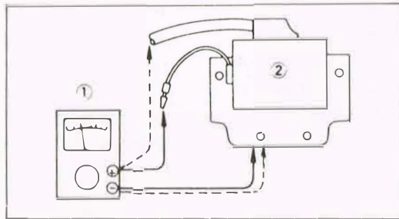
1. Primary coil resistance check 2. Secondary coil resistance check
