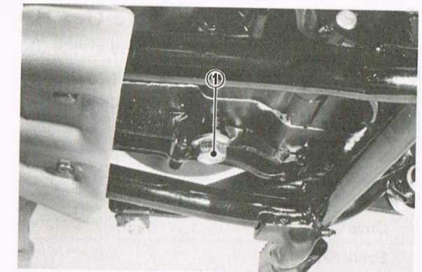
1. Drain plug
