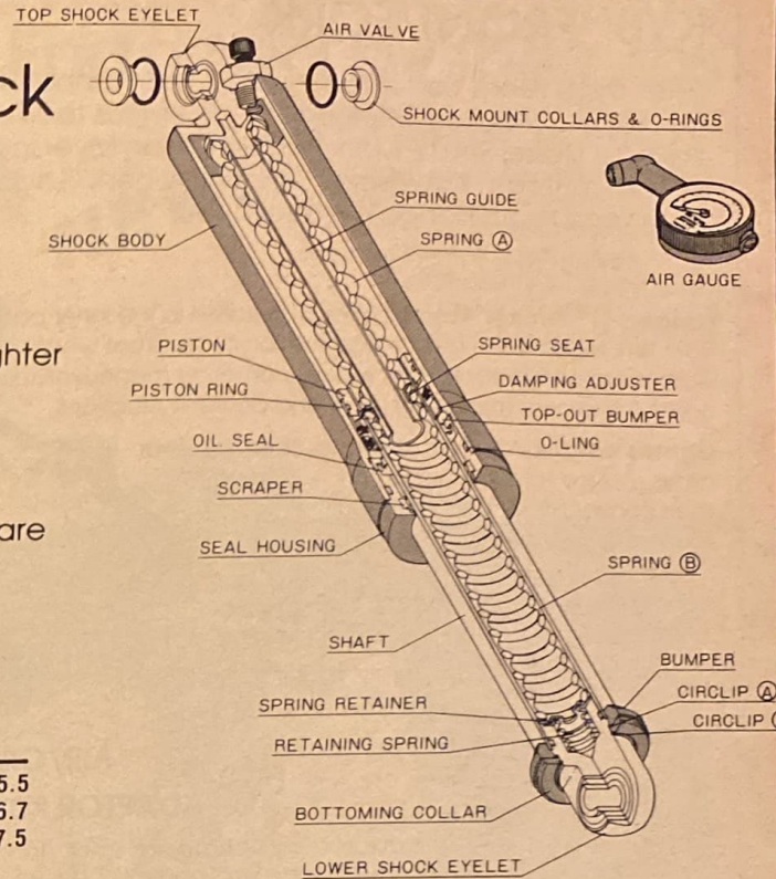
DIAGRAM OF SHOCK PARTS
