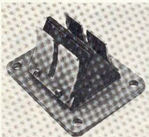
IT reed cage is identical to the YZ item, but piston thickness was increased to 2.0mm for greater durability.
