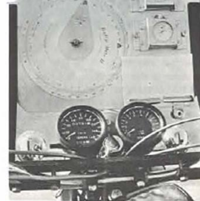
Just look at a special meter panel, which he has made all for himself. A disc calculator (left), watch (right top) and stop watch (right bottom).
