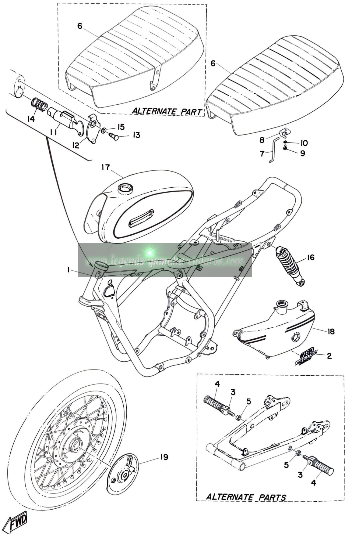
Fig. 4 FRAME, SEAT & TANK
