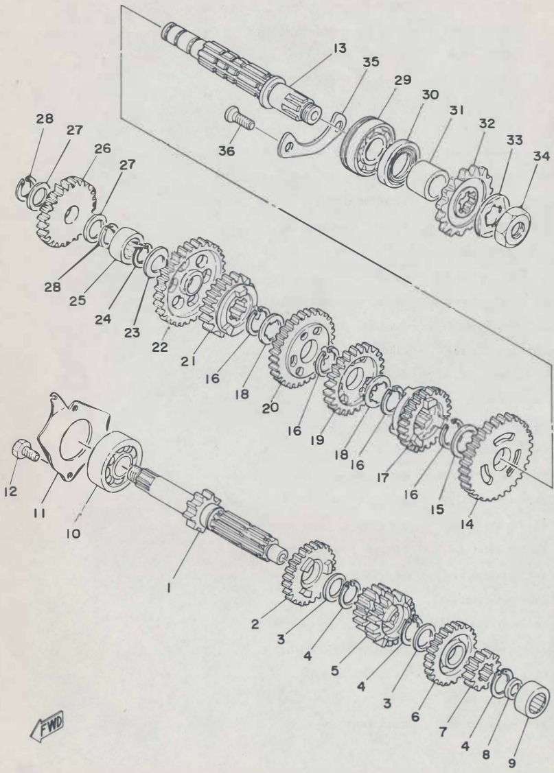
Fig. 5 TRANSMISSION
