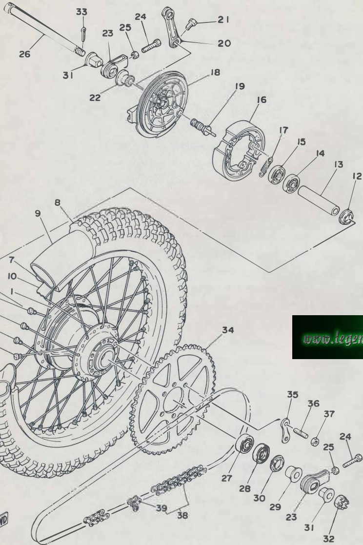
Fig. 26 REAR WHEEL
