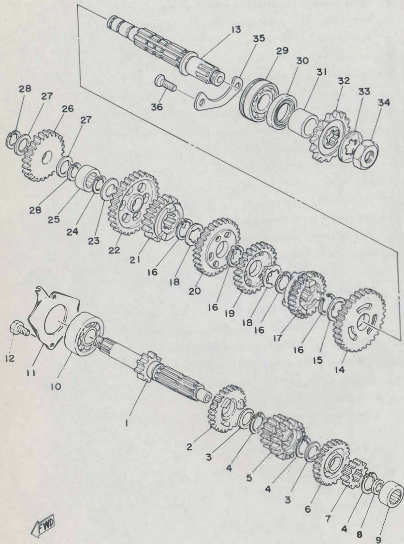
Fig. 5 TRANSMISSION
