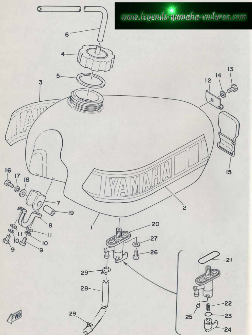
Fig. 23 FUEL TANK
