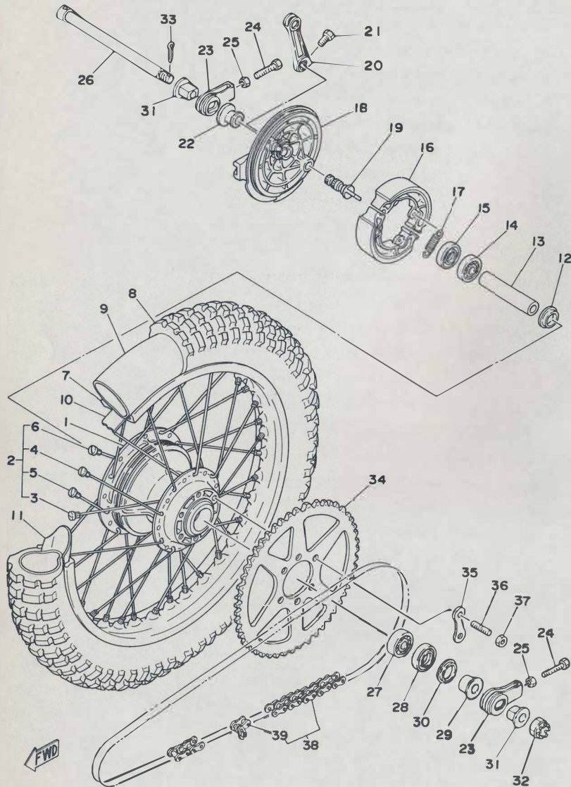
Fig. 26 REAR WHEEL
