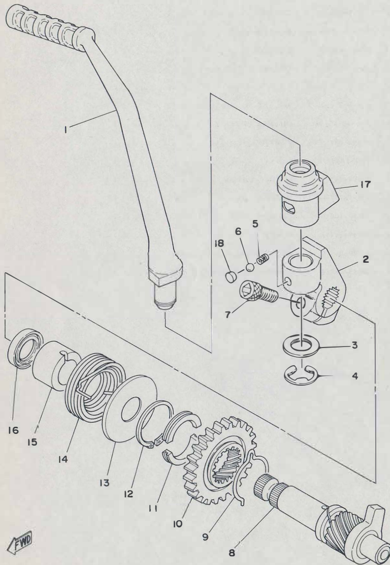
Fig. 8 KICK STARTER
