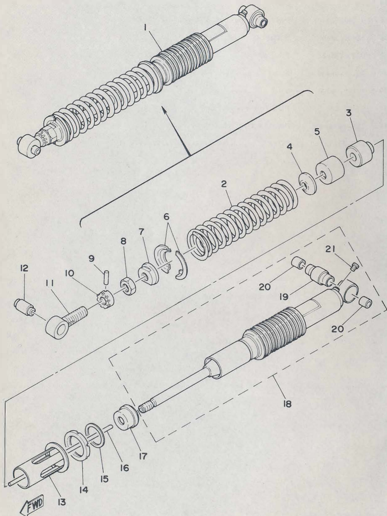
Fig. 15 REAR CUSHION (Except IRAN)
