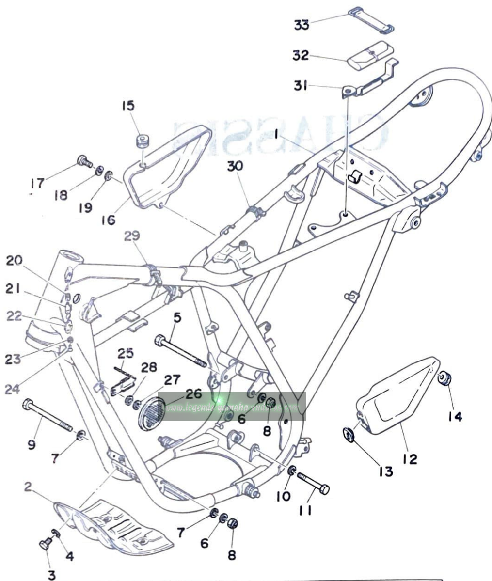
Fig. 15 FRAME · SIDE COVER
