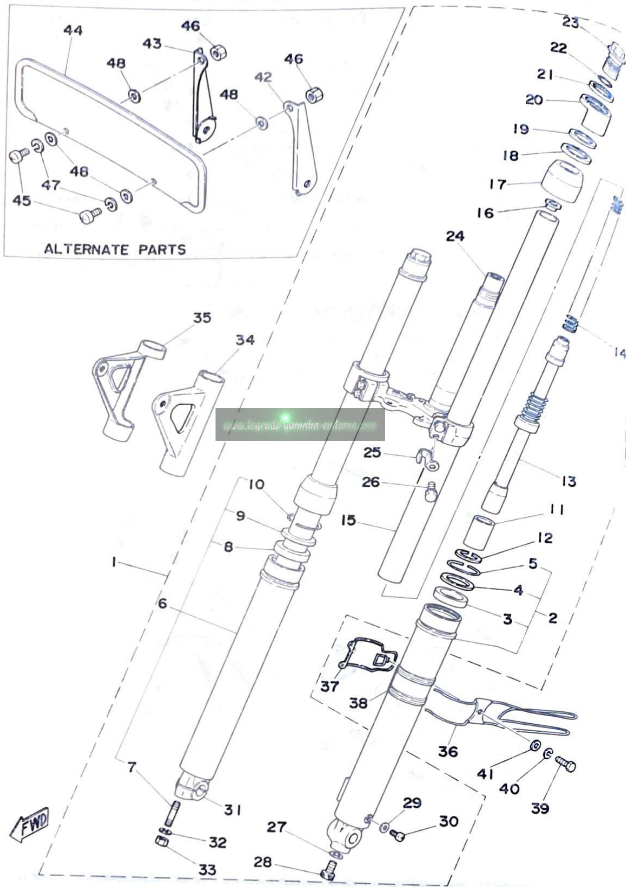
Fig. 19 FRONT FORK
