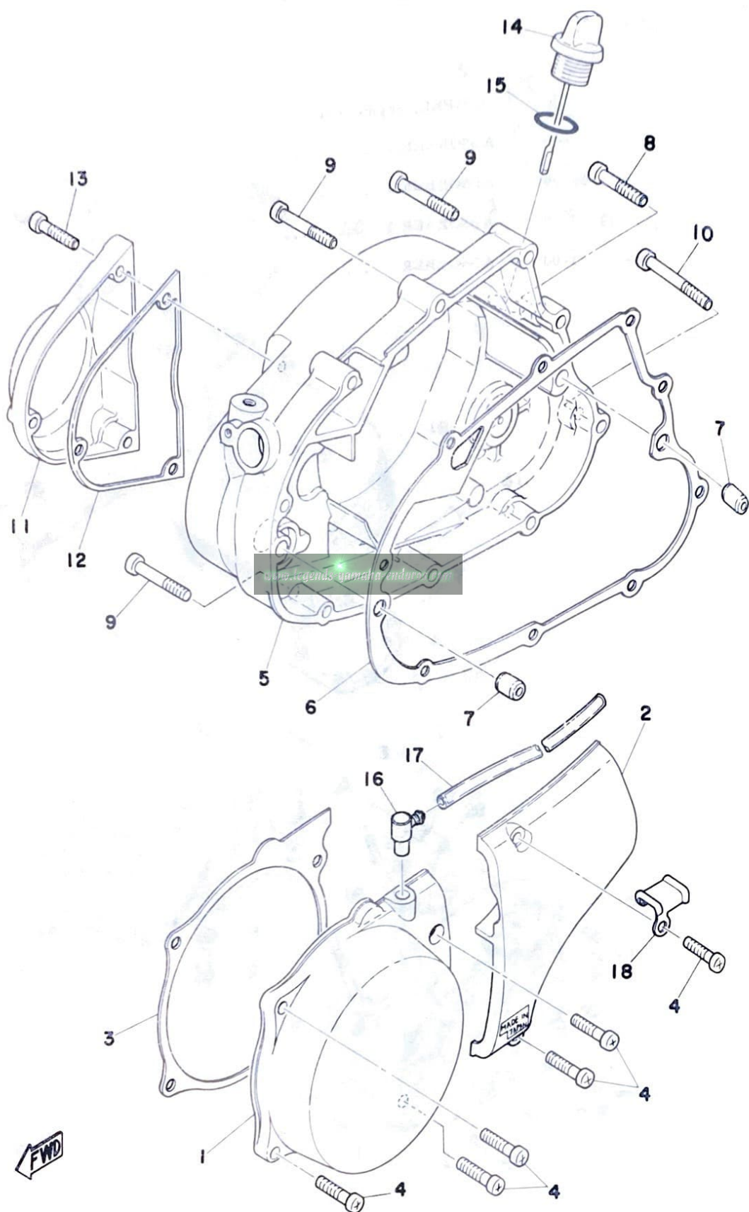
Fig. 2 CRANKCASE COVER
