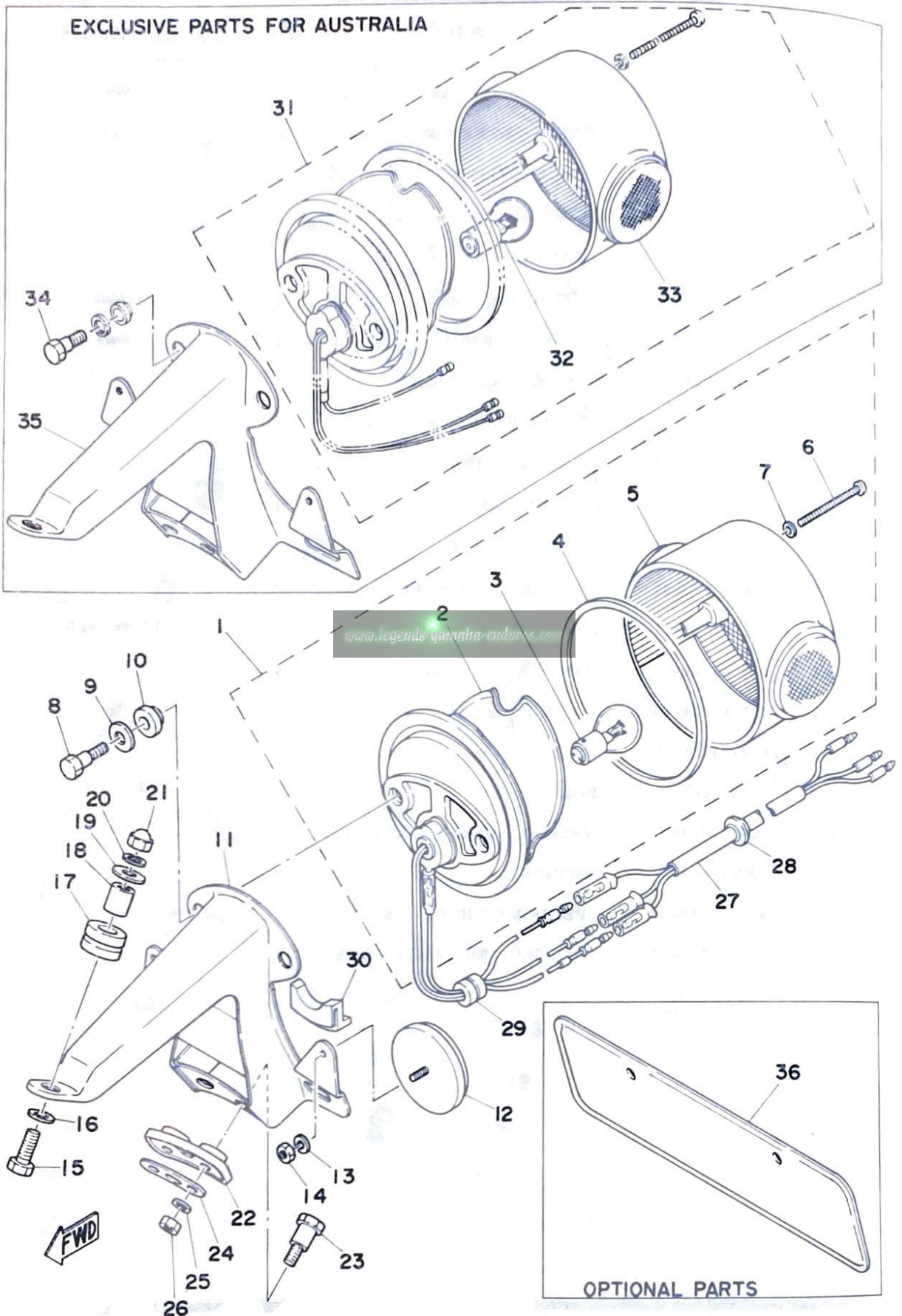
Fig. 29 TAIL LAMP
