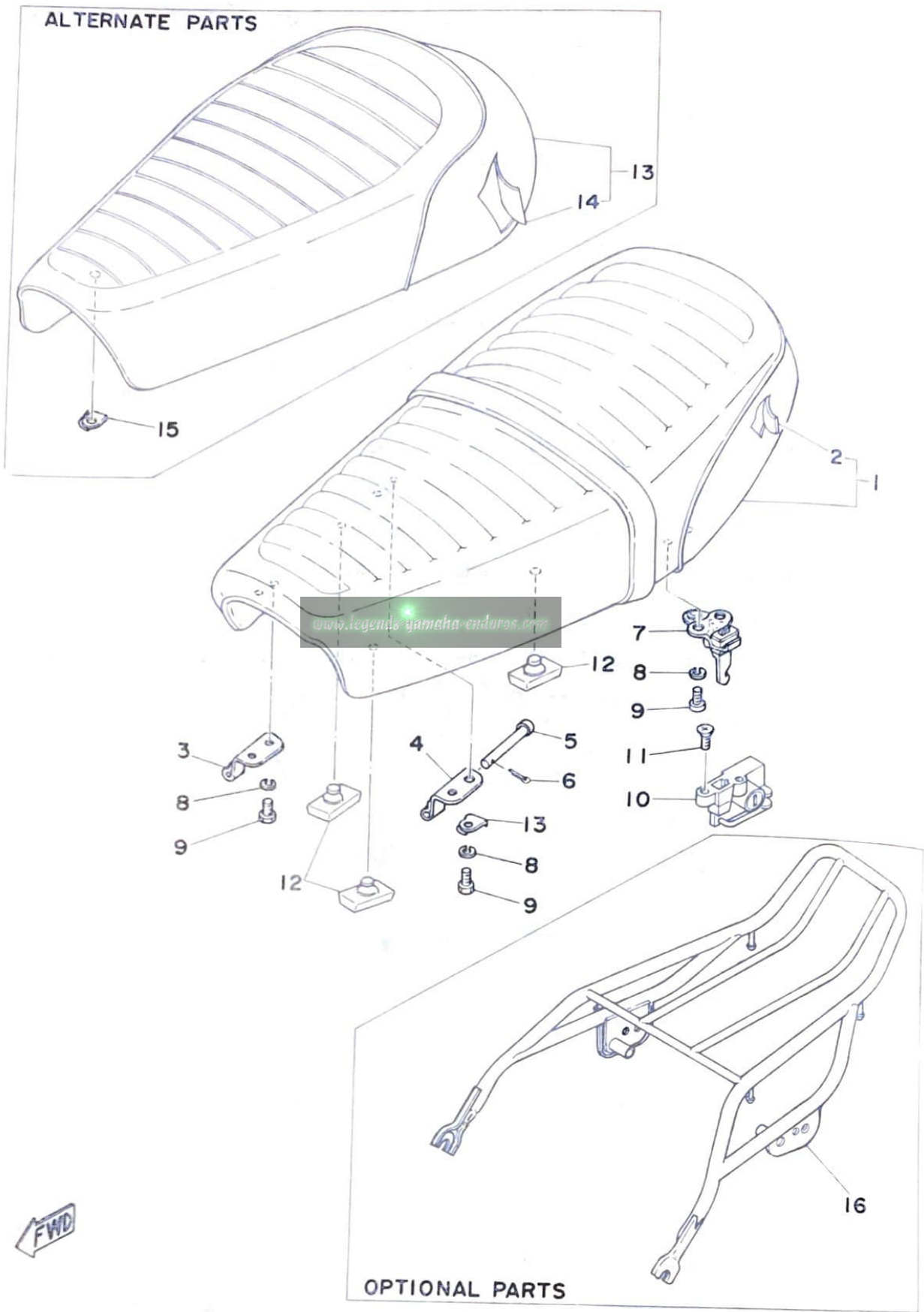
Fig. 24 SEAT
