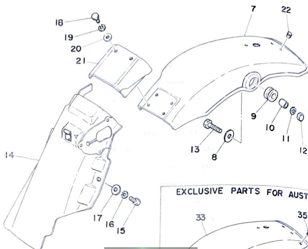
Fig. 18 FRONT FENDER · REAR FENDER
