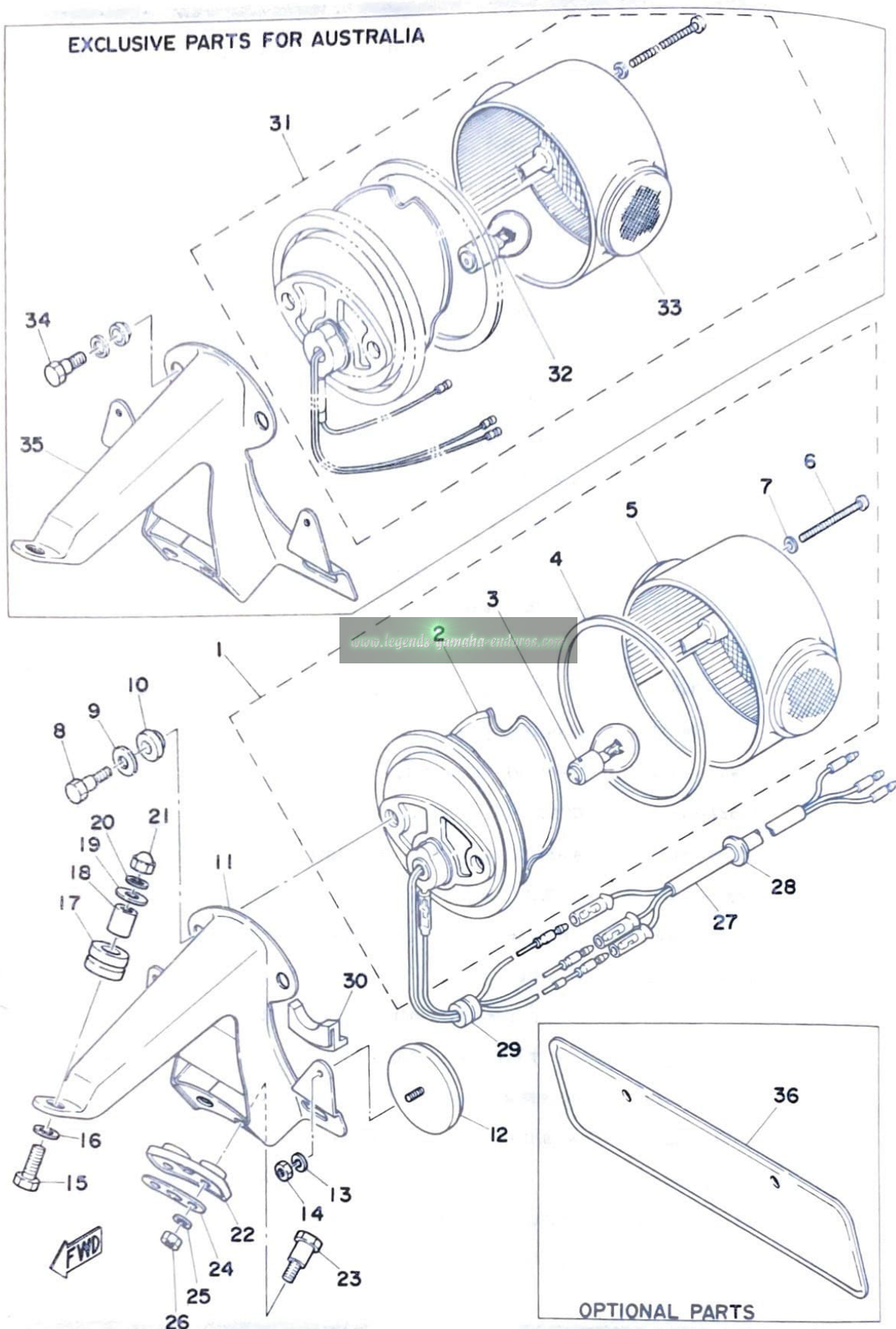
Fig. 29 TAIL LAMP
