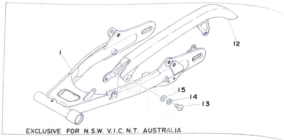
Fig.16 REAR ARM · REAR CUSHION · CHAIN CASE
