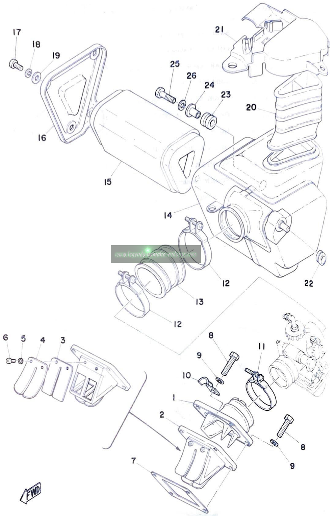
Fig. 10 INTAKE
