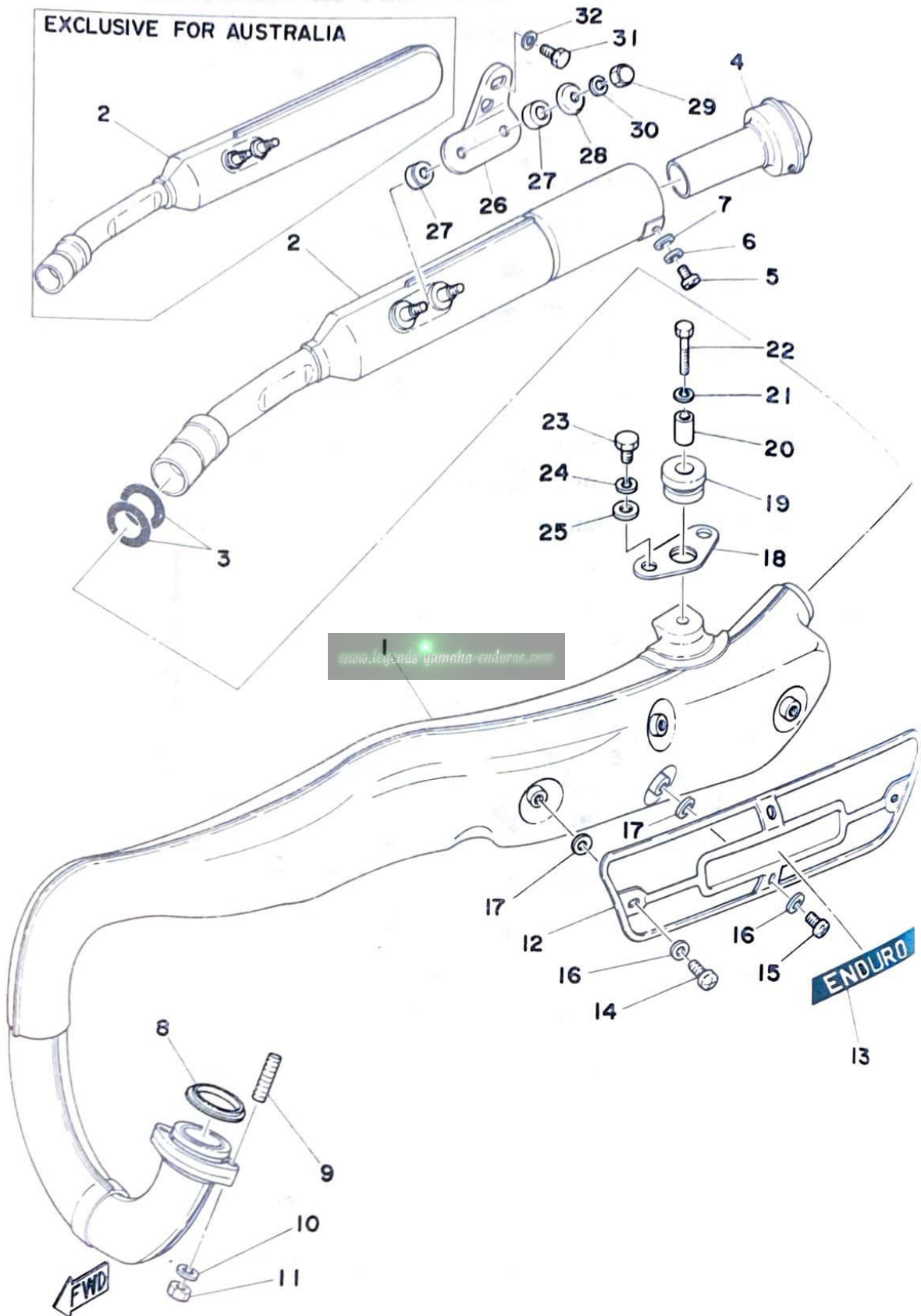
Fig. 12 EXHAUST
