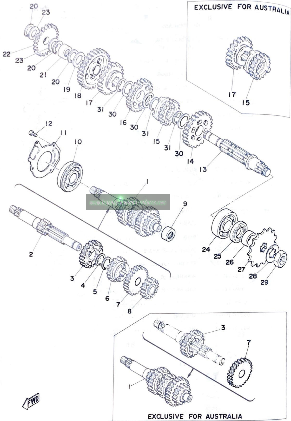
Fig. 5 TRANSMISSION
