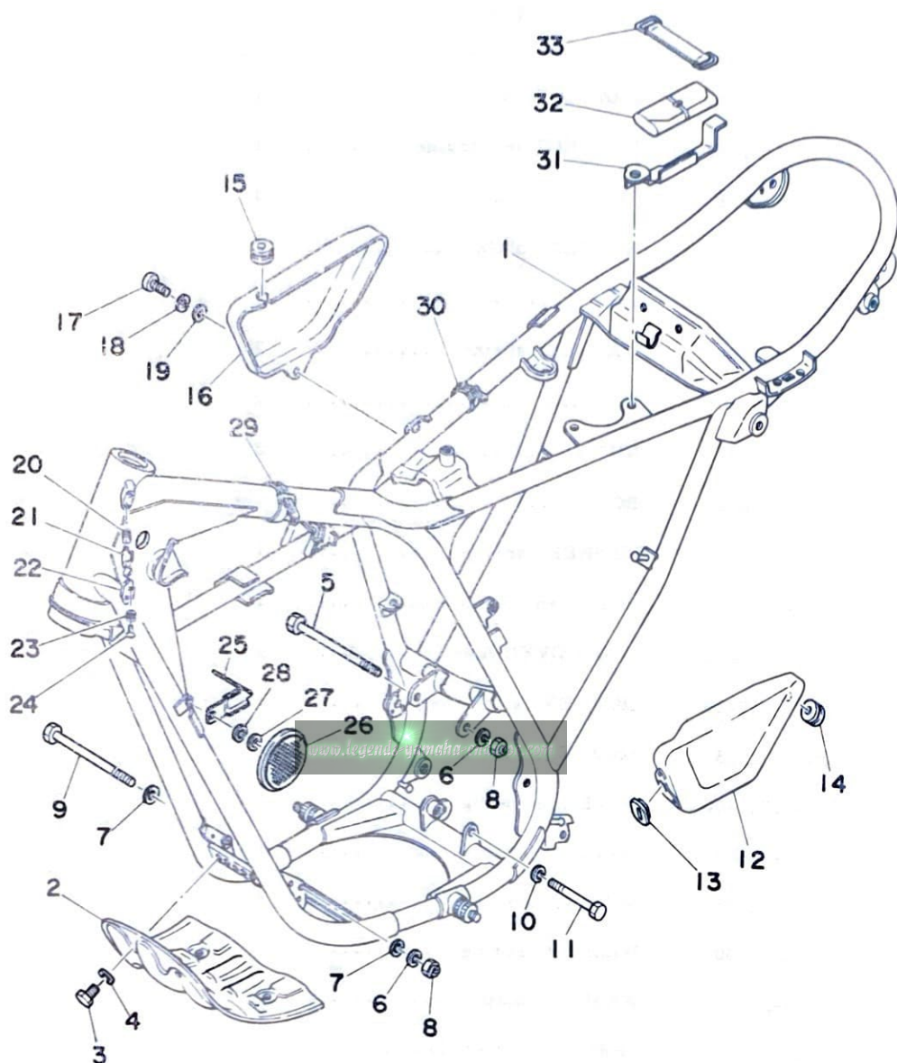
Fig. 15 FRAME · SIDE COVER
