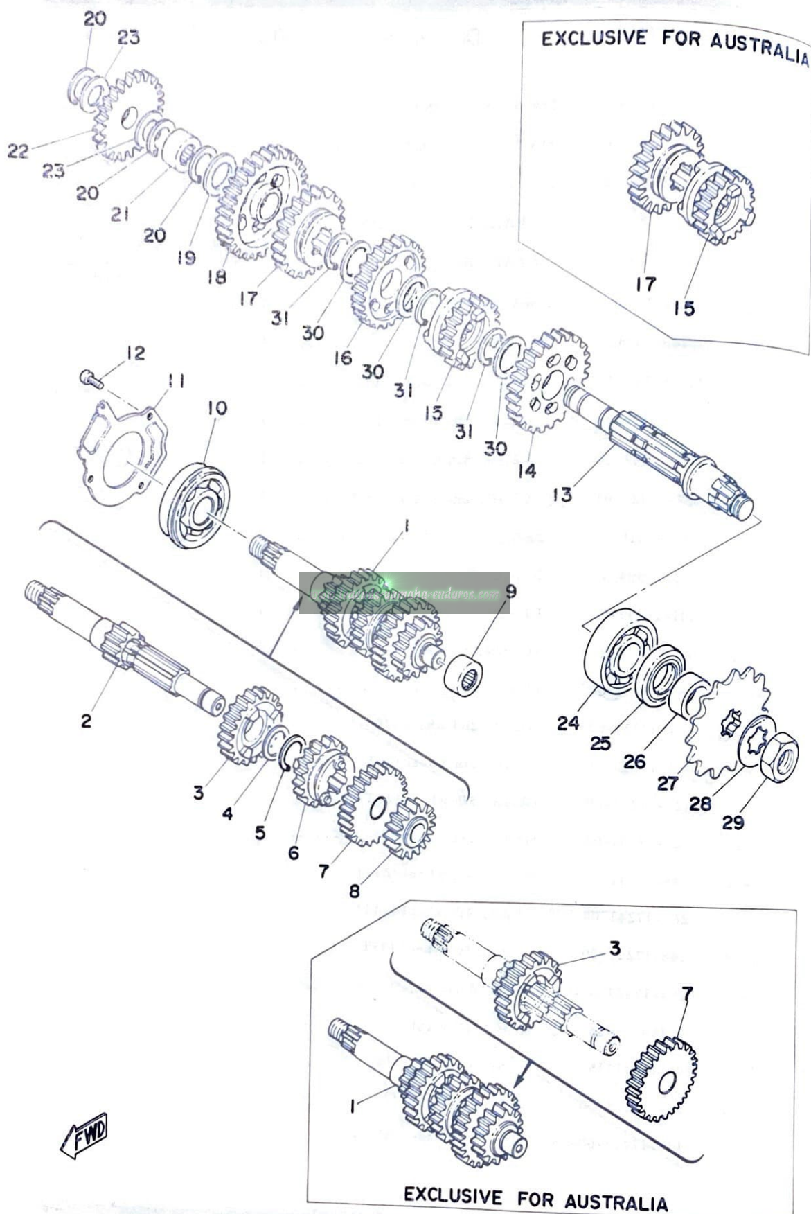
Fig. 5 TRANSMISSION
