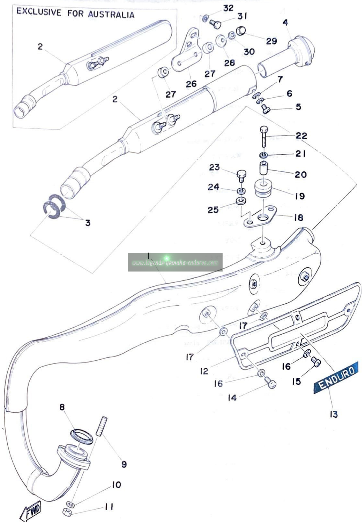
Fig. 12 EXHAUST
