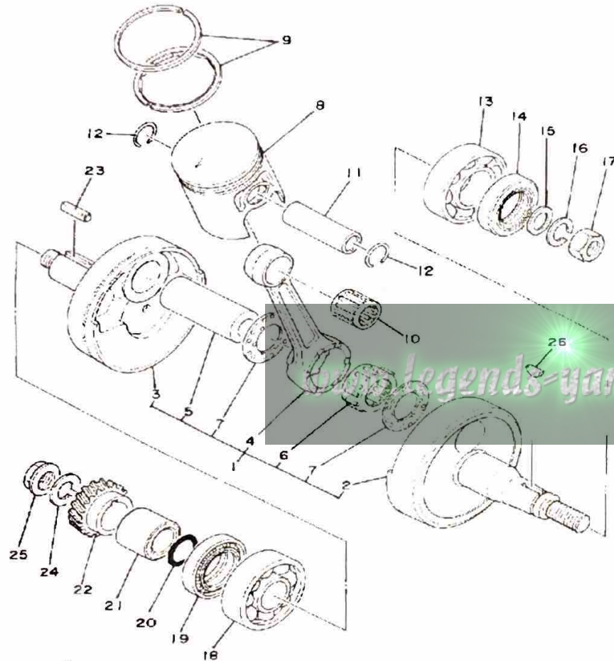
SPECIAL SERVICE TOOLS TLU-90900-57-01 CRANKSHAFT INSTALLING SET
