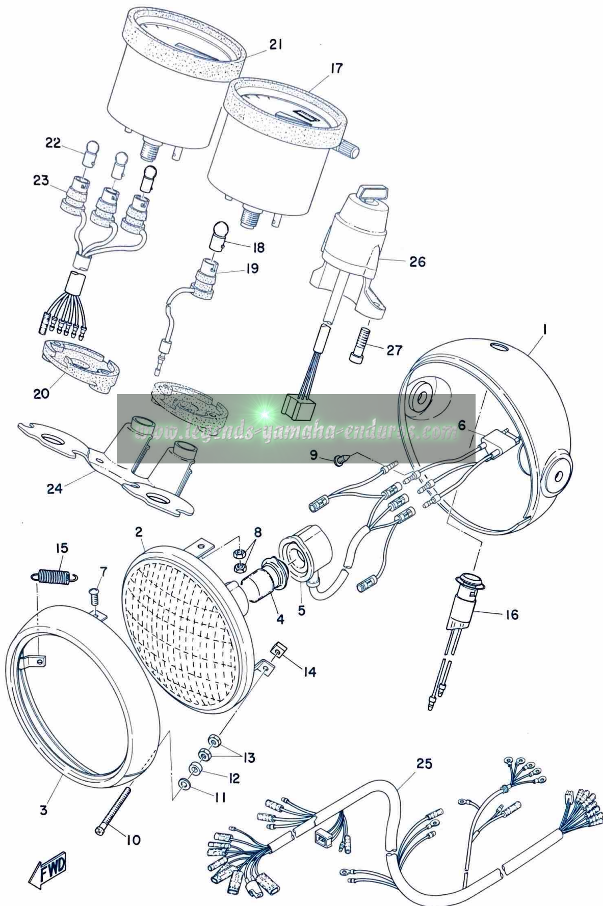
Fig. 4 HEAD LAMP, SPEEDOMETER & TACHOMETER
