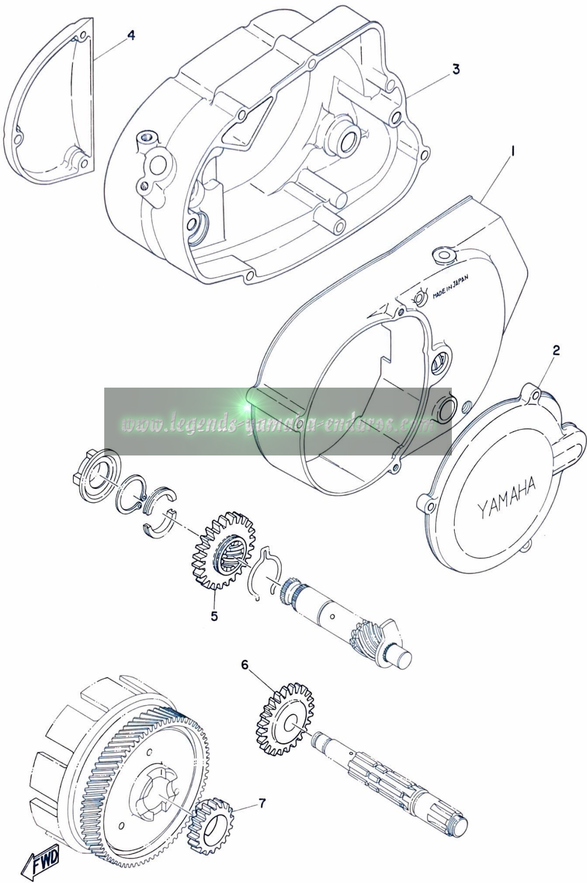
Fig. 1 ENGINE
