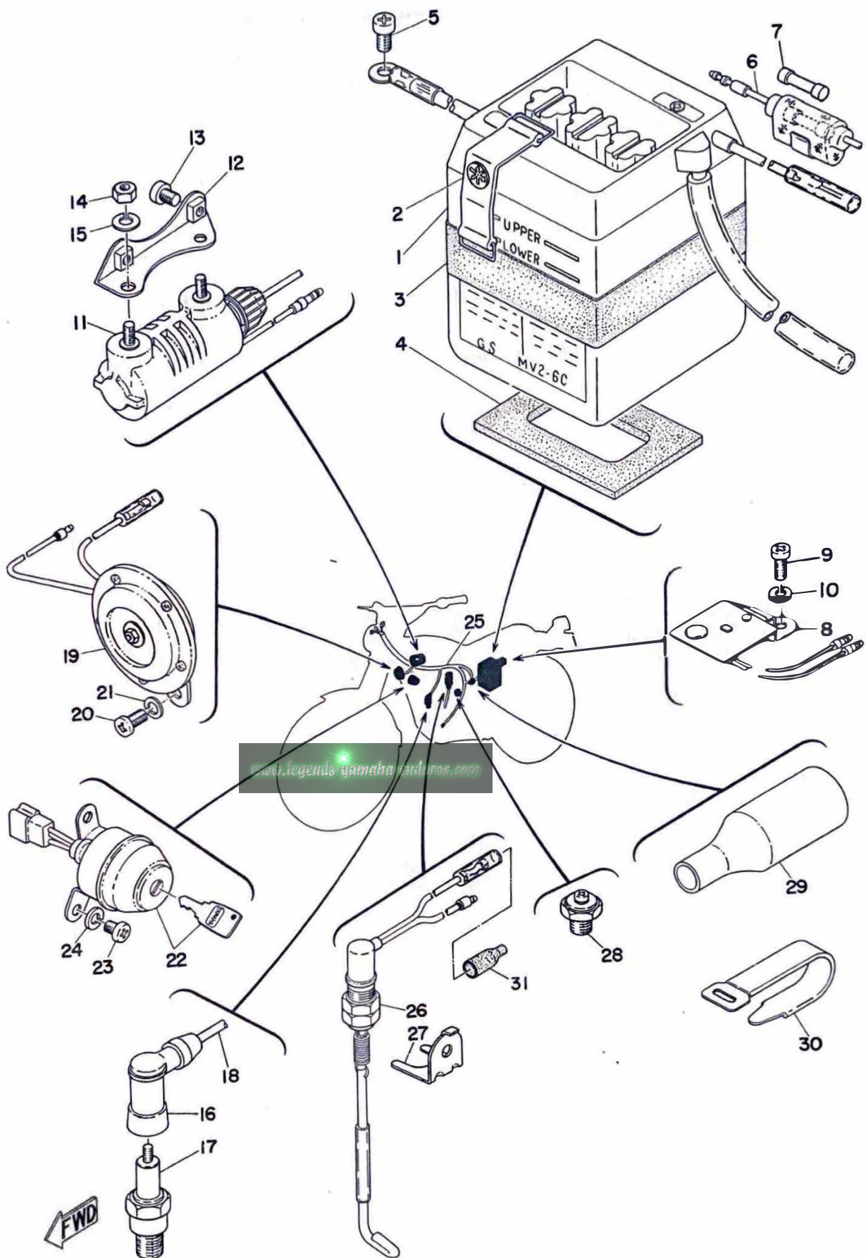
Fig. 27 ELECTRICAL
