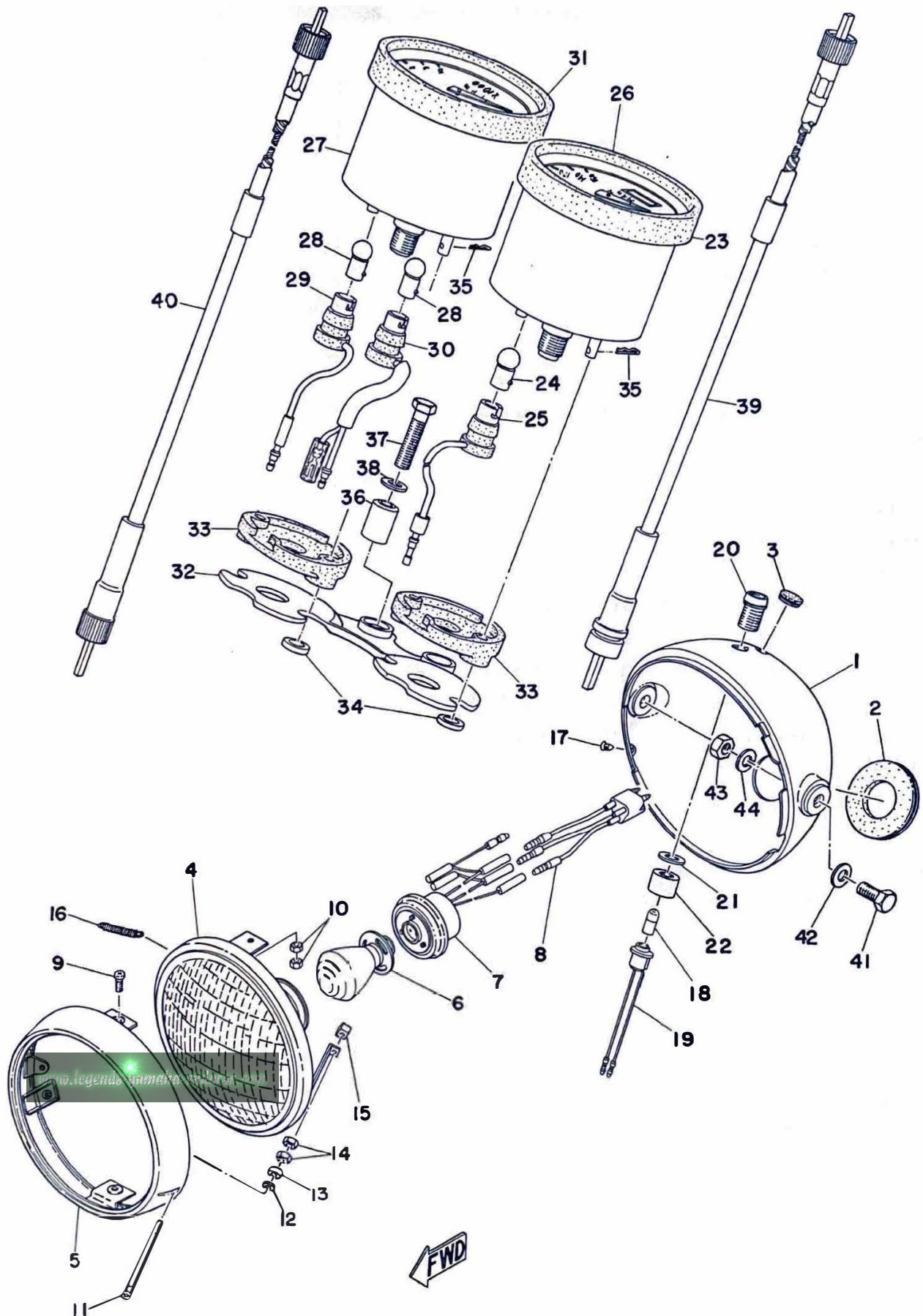
Fig. 25 HEAD LAMP, SPEEDOMETER & TACHOMETER
