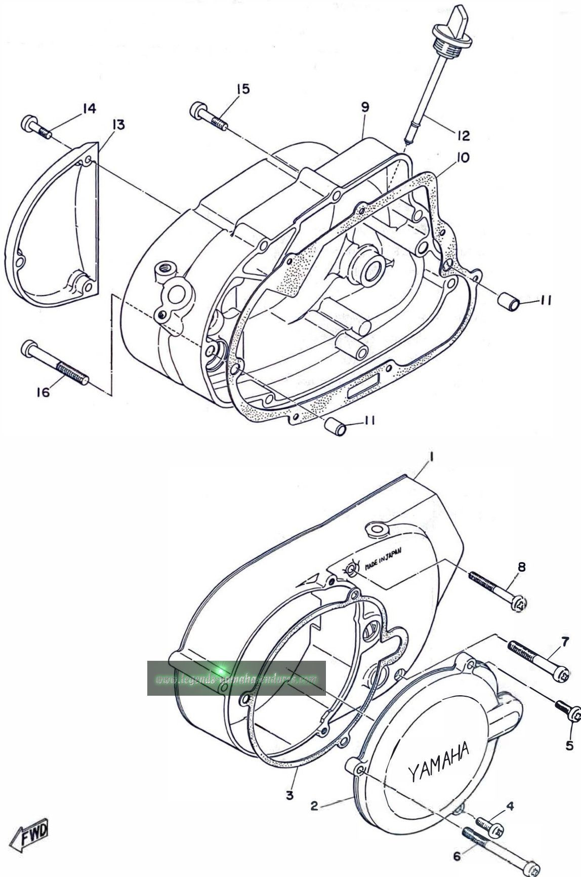
Fig. 2 CRANKCASE COVER
