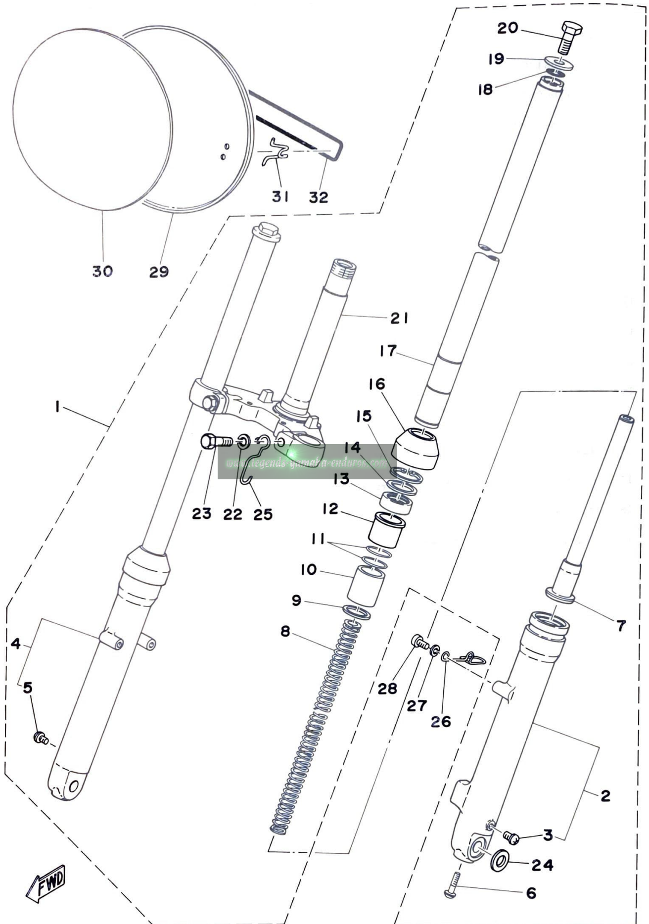
Fig. 17 FRONT FORK
