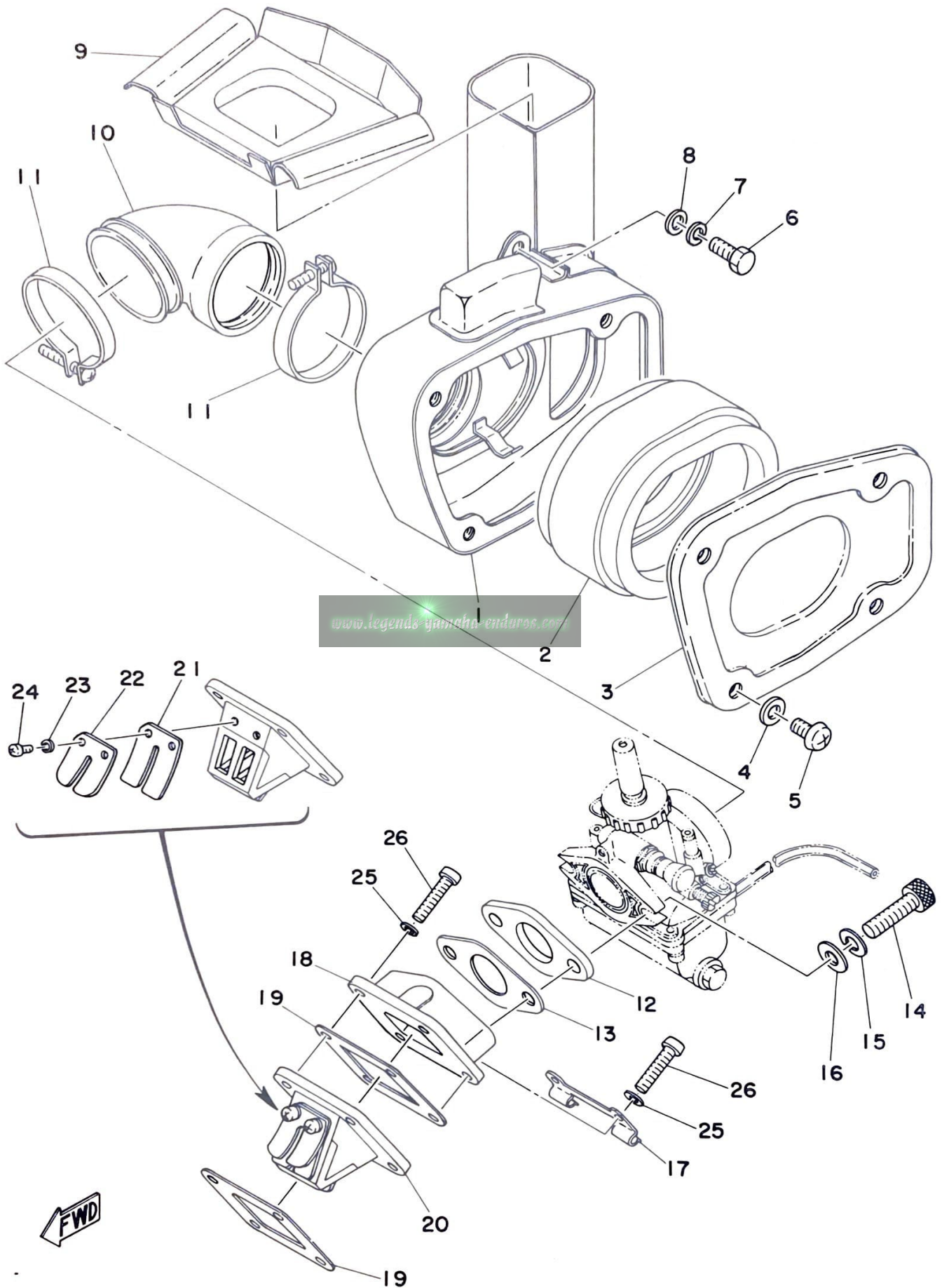
Fig. 9 INTAKE
