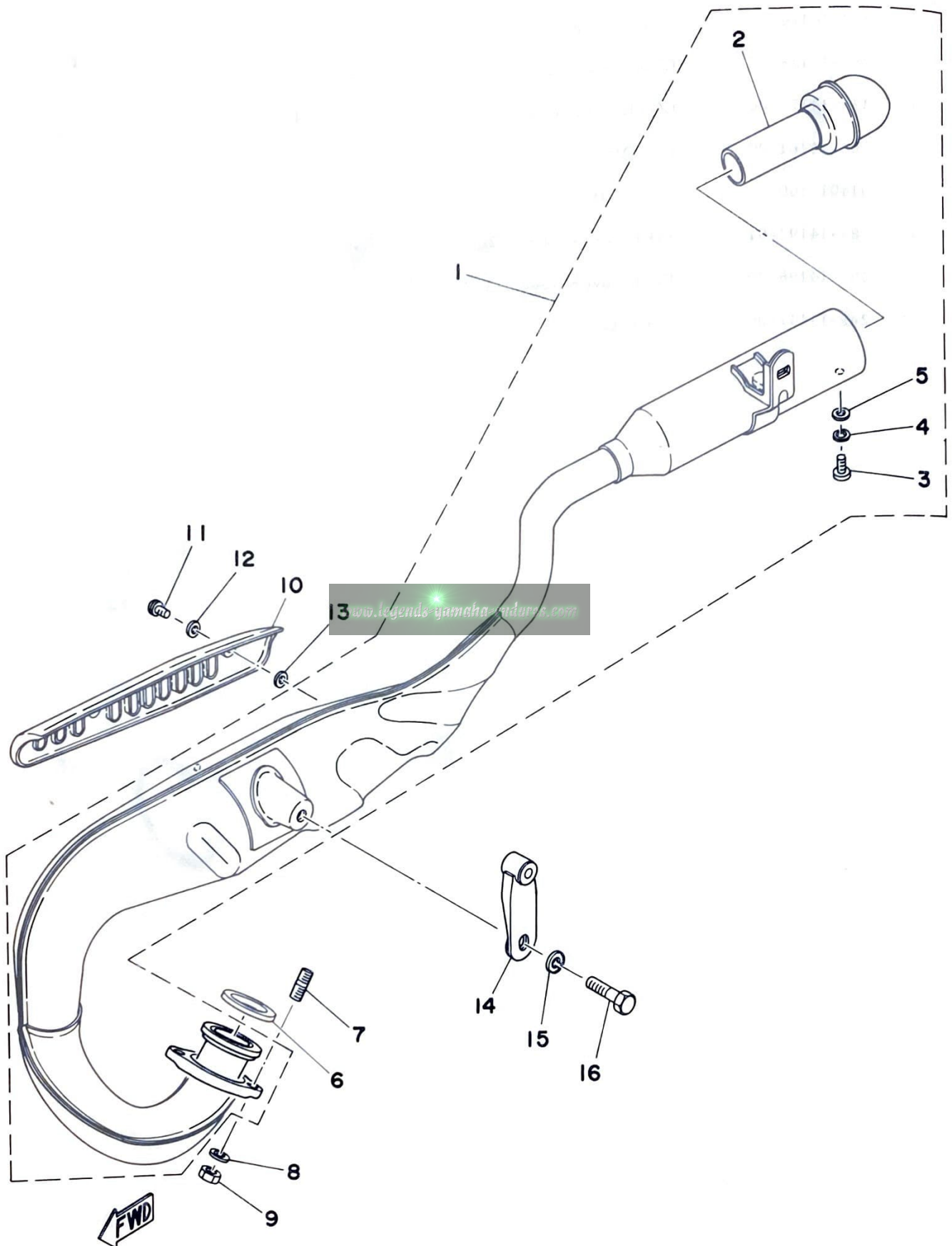
Fig. 11 EXHAUST
