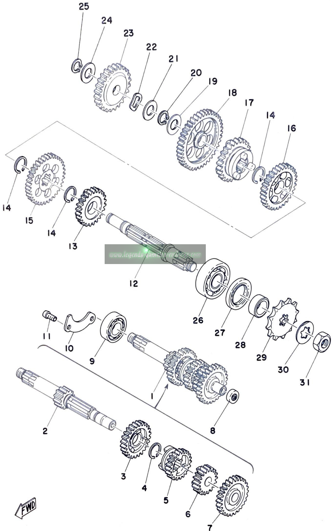
Fig. 5 TRANSMISSION
