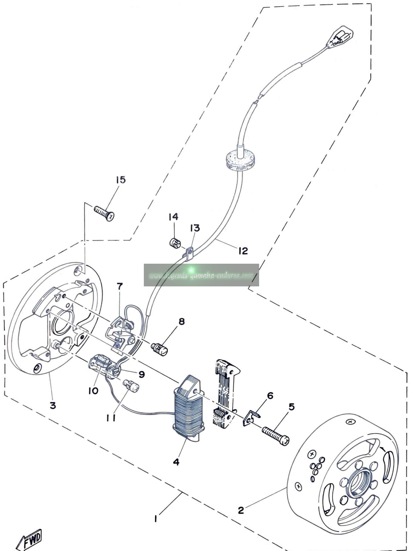
Fig. 12 FLYWHEEL MAGNETO
