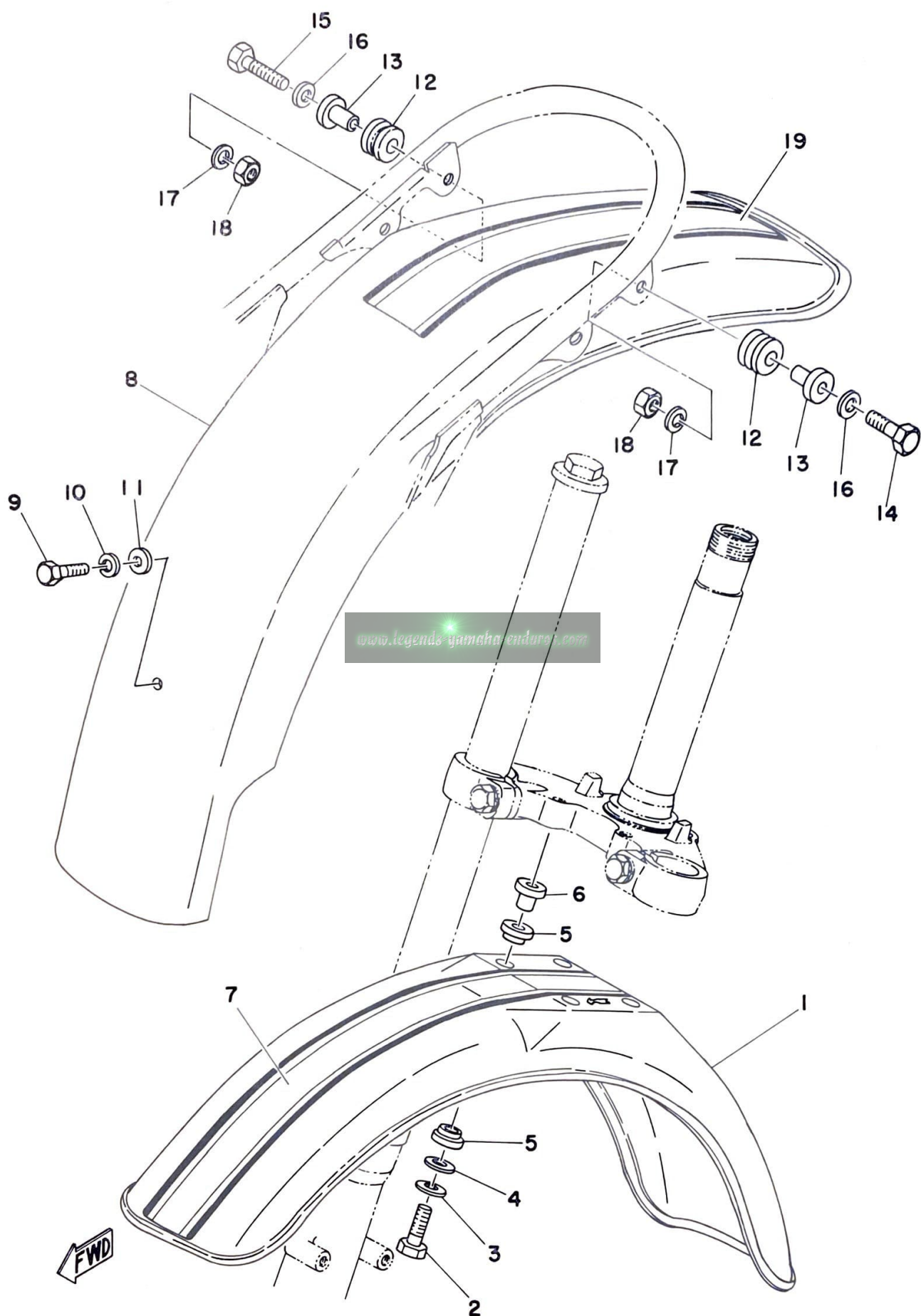
Fig. 16 FRONT FENDER · REAR FENDER
