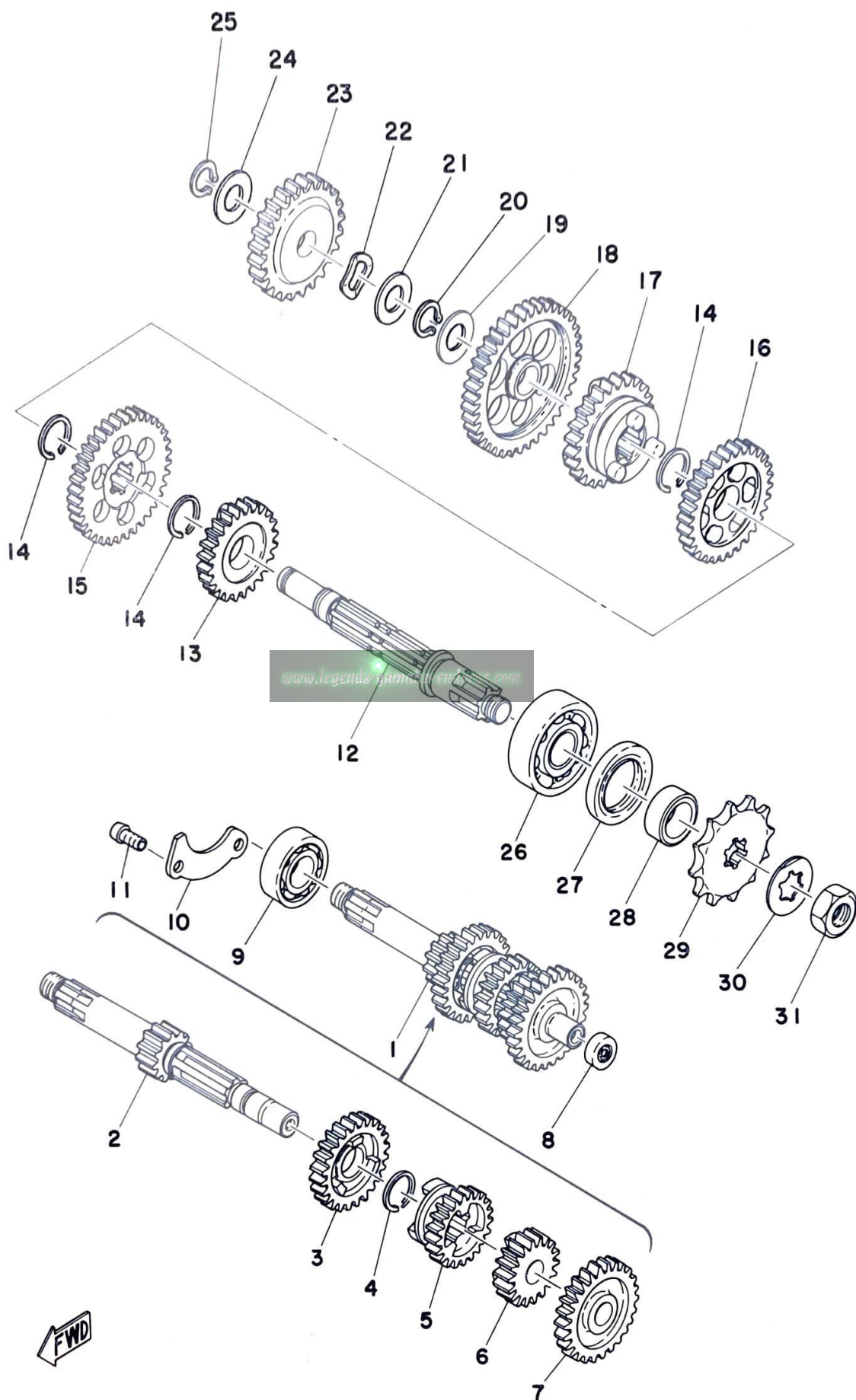
Fig. 5 TRANSMISSION
