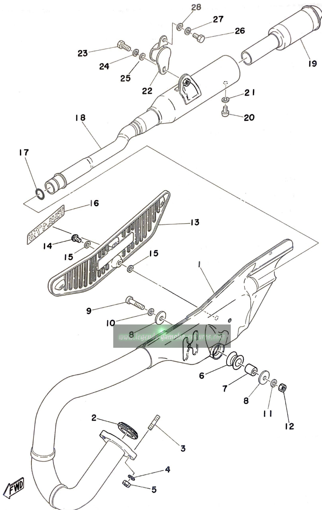
Fig. 12 EXHAUST
