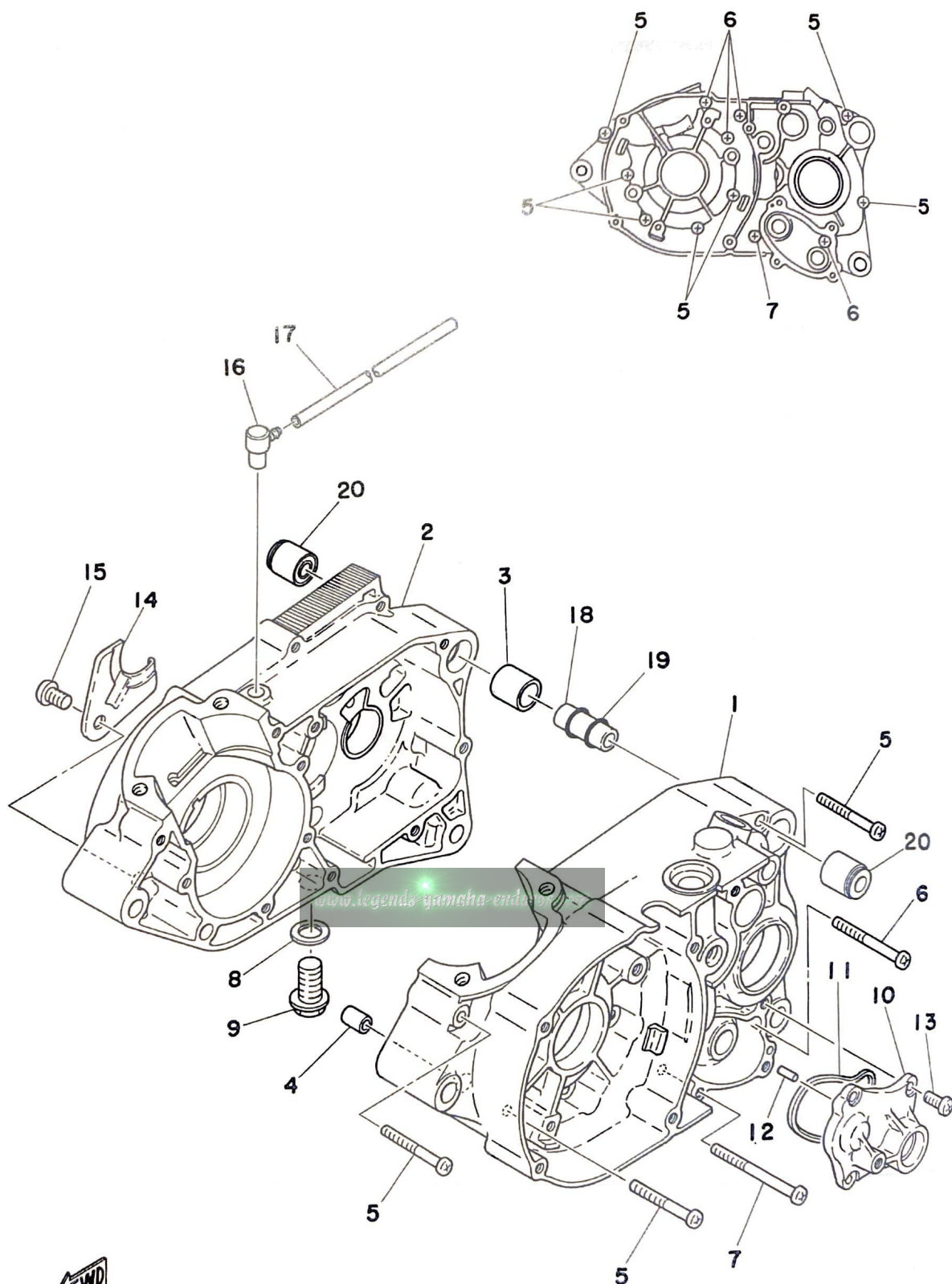
Fig. 2 CRANKCASE
