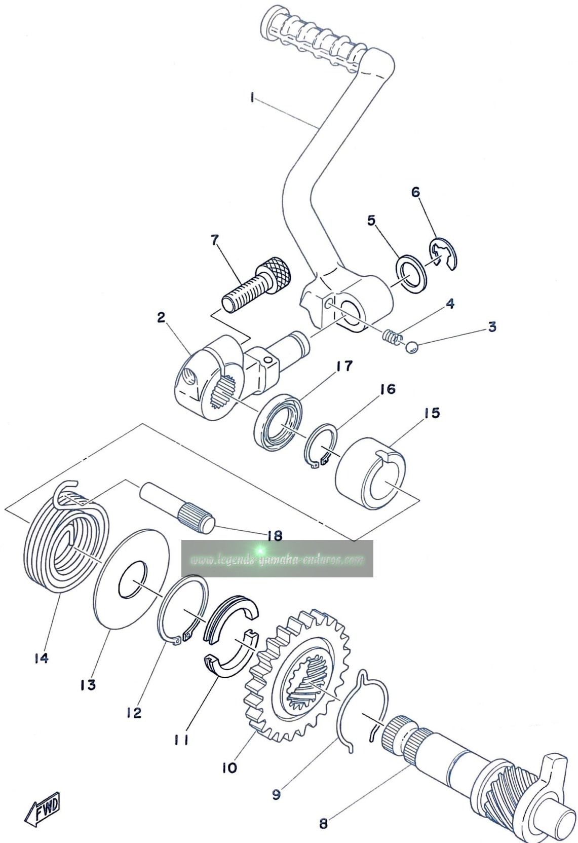
Fig. 9 KICK STARTER
