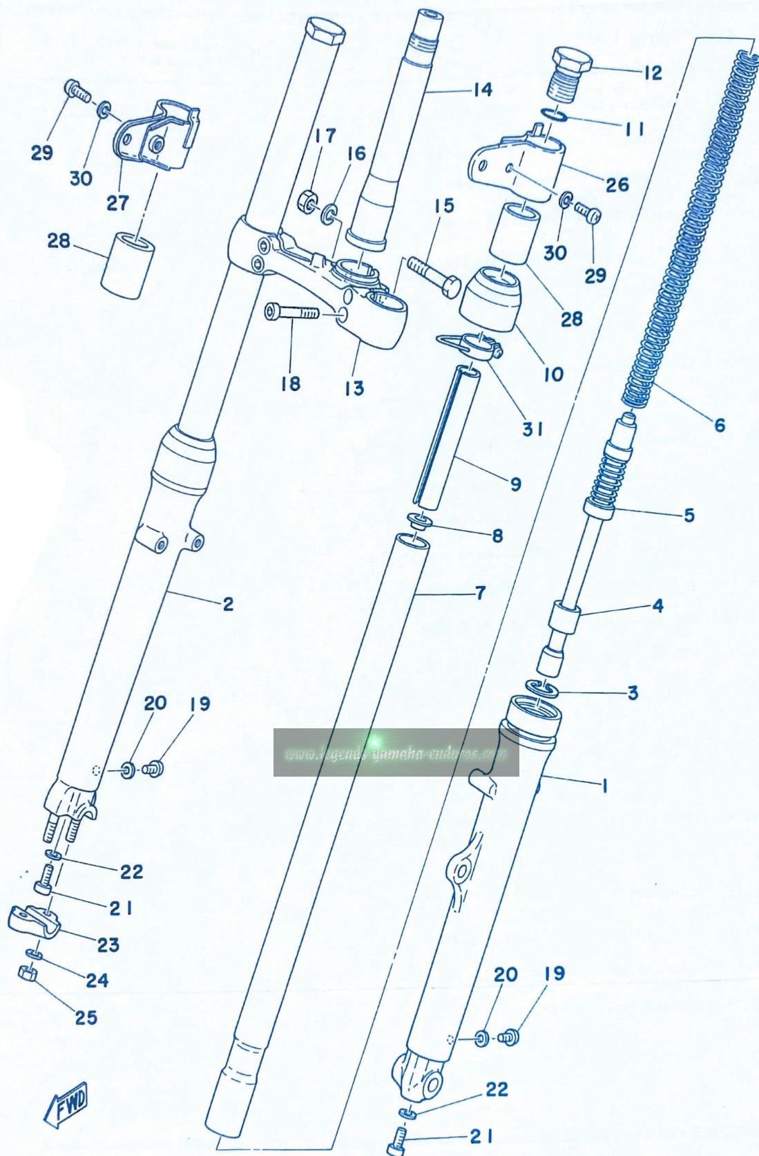
Fig. 19 FRONT FORK
