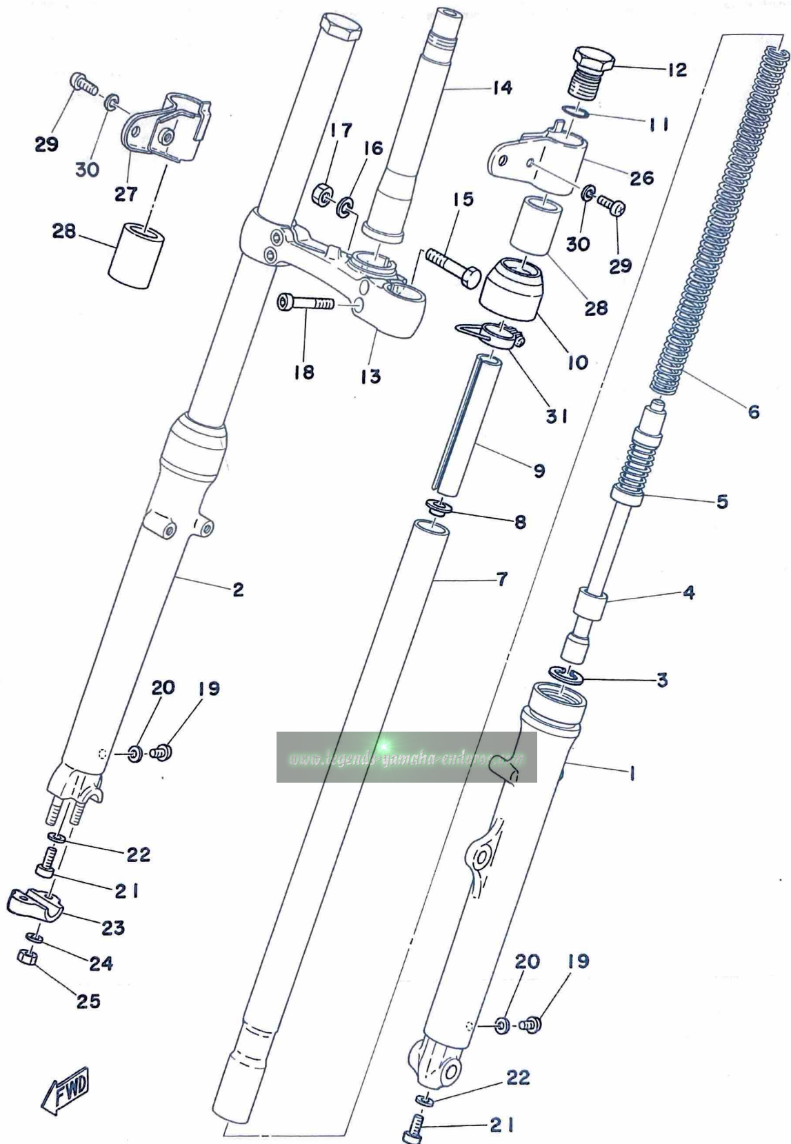
Fig. 19 FRONT FORK
