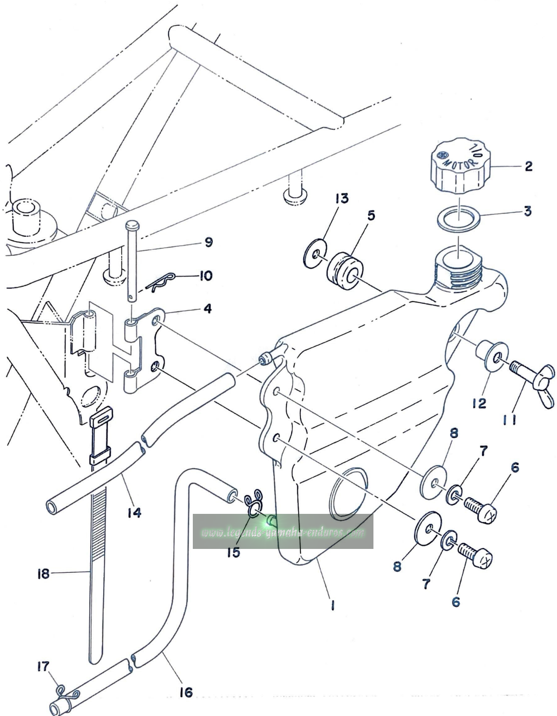
Fig. 23 OIL TANK
