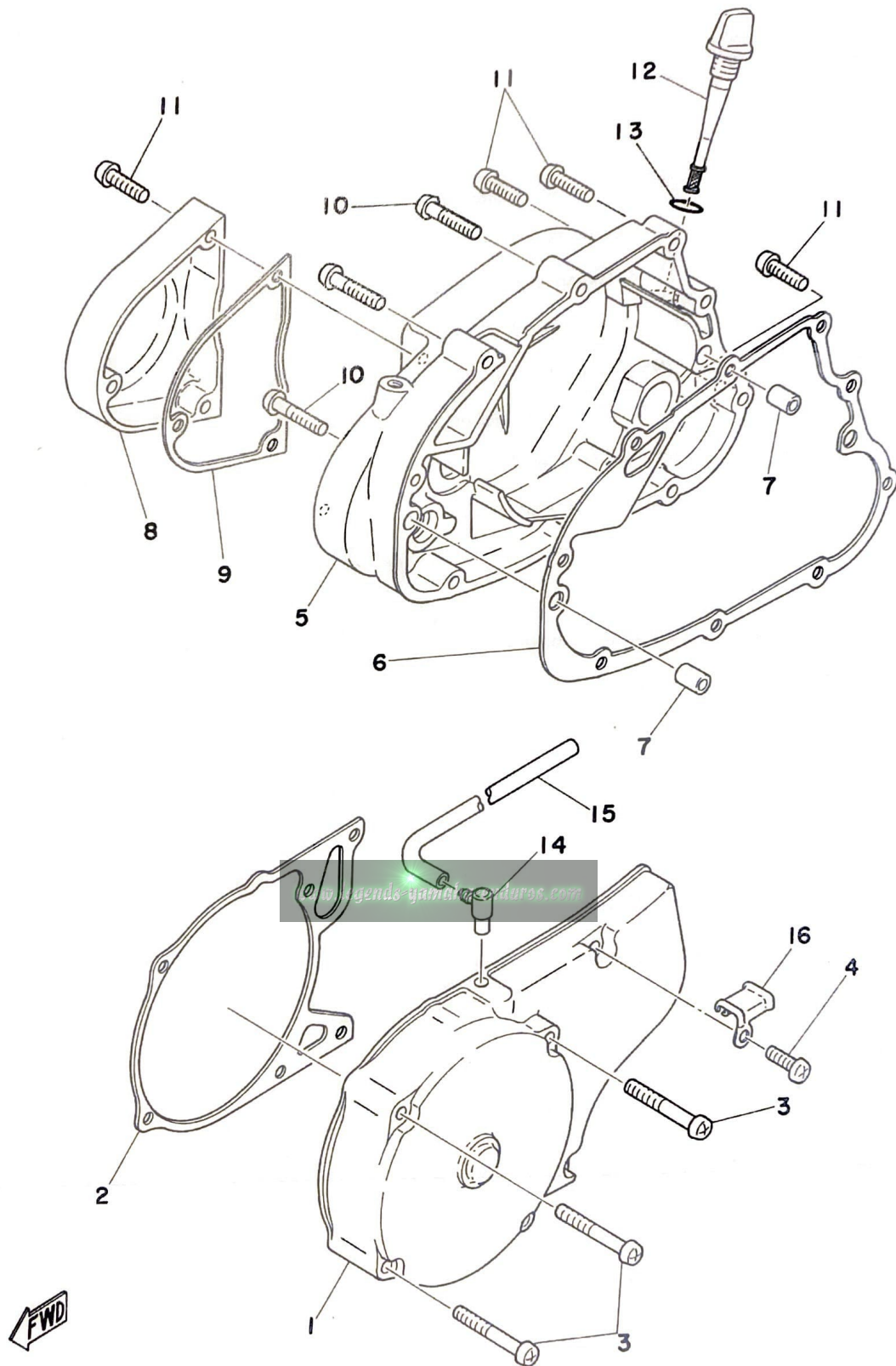
Fig. 3 CRANKCASE COVER
