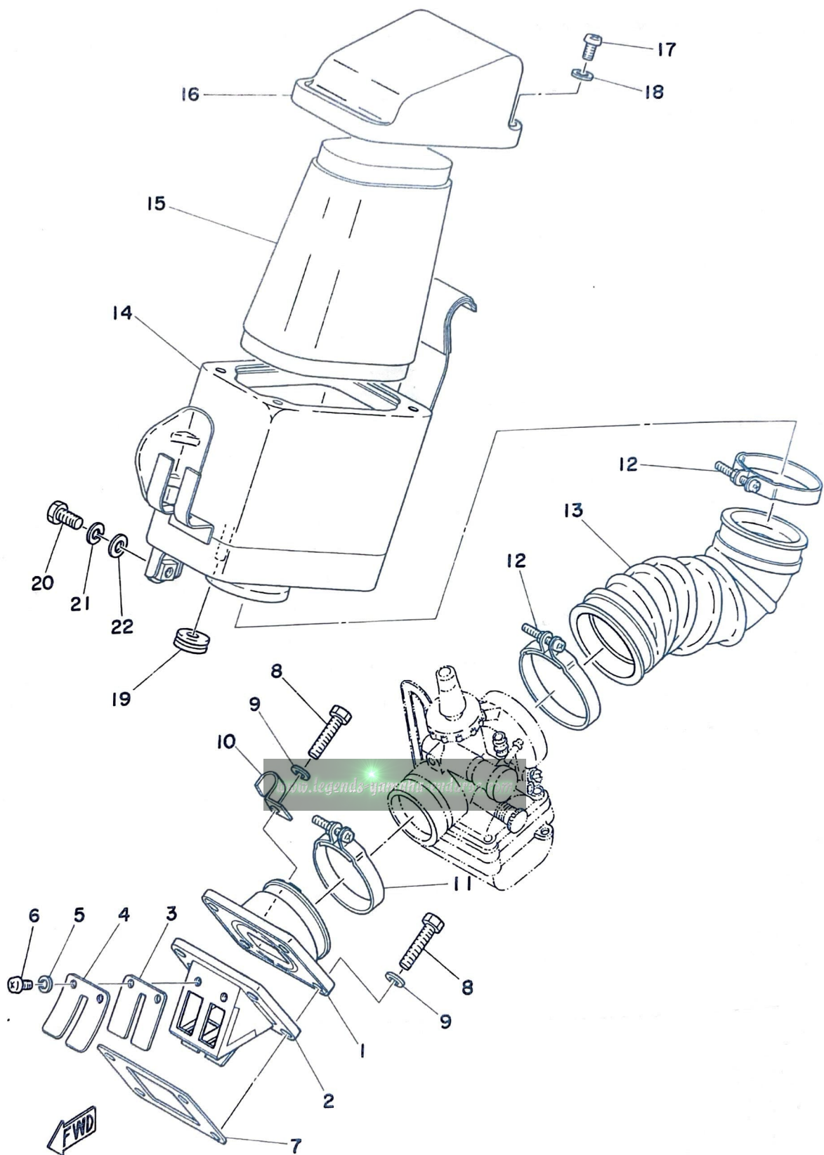
Fig. 10 INTAKE
