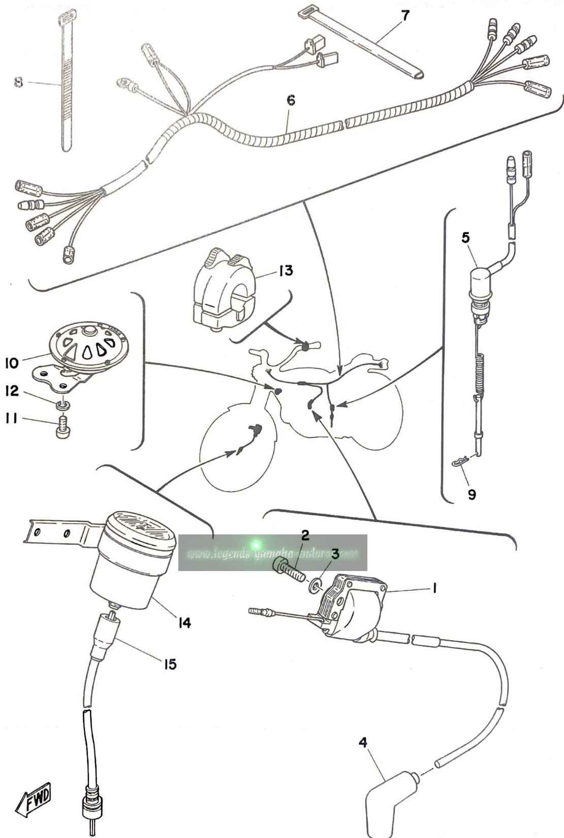
Fig. 29 ELECTRICAL
