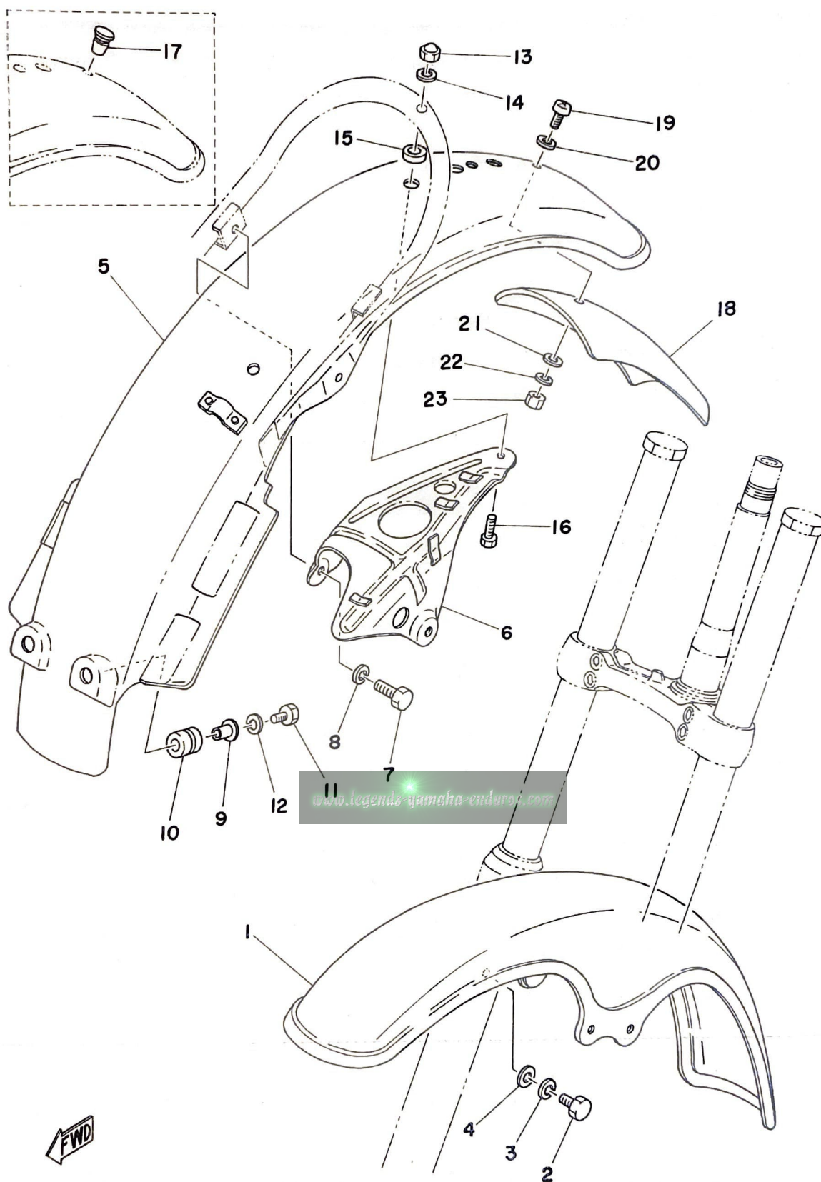
Fig. 18 FRONT FENDER · REAR FENDER
