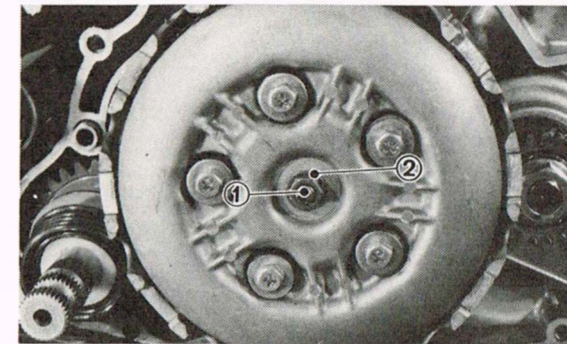
1. Adjuster 1. Adjusting screw 2. Lock nut 2. Erou de blocage
