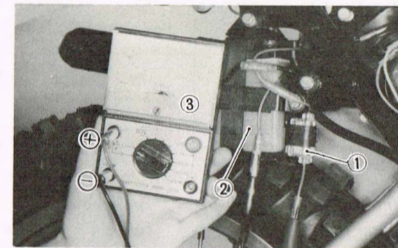
1. Fuse 2. Battery 3. Set the tester in "DC. A-5" position.
