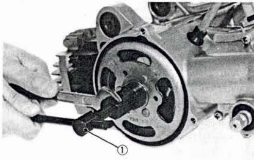
1. Flywheel puller
