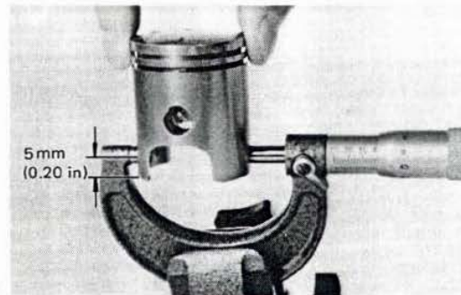
Piston diameter
